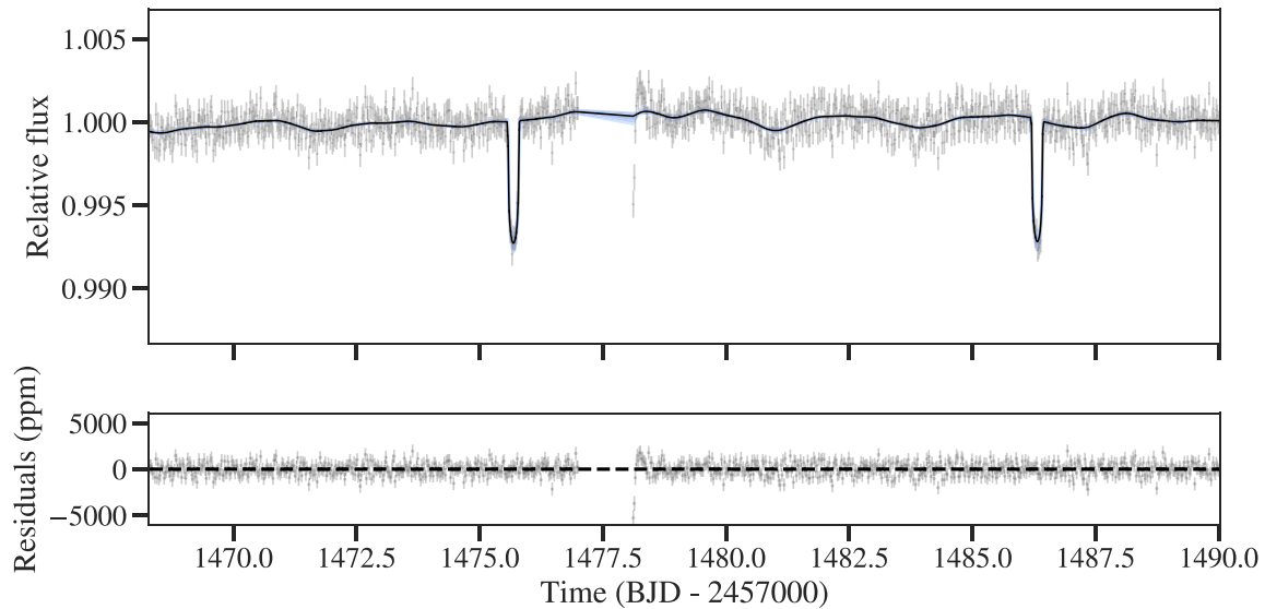
Figure 2. The top panel corresponds to the TESS 30 minute cadence light curve of TOI-892 generated through tesseract from the full-frame images of Sector 6. The solid line corresponds to the model generated from the posterior parameters of the analysis presented in Section 3. The bottom panel shows the residuals between the TESS light curve and the model.
