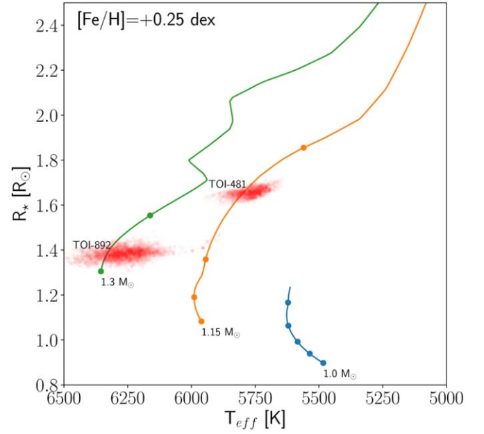
Figure 6. Posterior distributions for the effective temperature and stellar radius of TOI-481 and TOI-892 (red clumps). The lines represent PARSEC stellar evolutionary tracks for stellar masses of 1 M_{\odot} (blue), 1.15 M_{\odot} (orange), and 1.3 M_{\odot} (green). A metallicity of [Fe/H] = +0.25 is assumed for the three evolutionary tracks, and the circles from bottom to top correspond of the ages of 1, 3, 5, and 7 Gyr.
