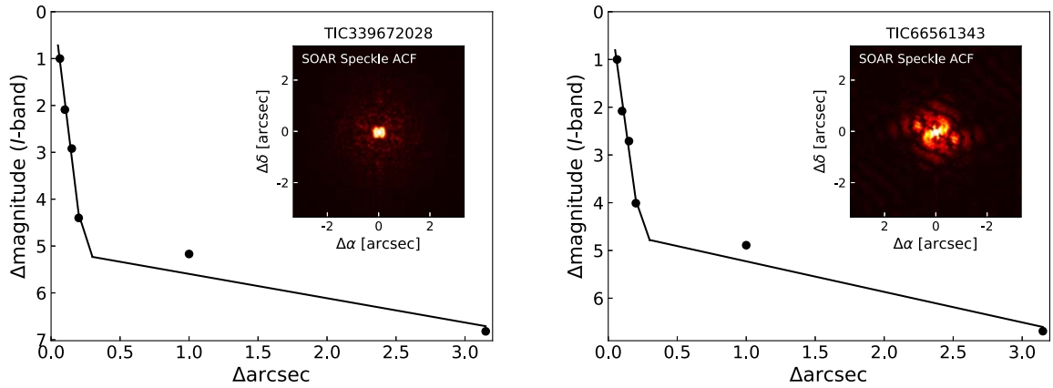
Figure 4. Contrast curve plots and autocorrelation functions from Speckle imaging in the I band using the HRcam at SOAR, for TOI-481 (left panel) and TOI-892 (right panel). The black points correspond to the 5\sigma contrast curve for each star. The solid line is the linear fit to the data for separations <0''.2 and >0''.2 .
