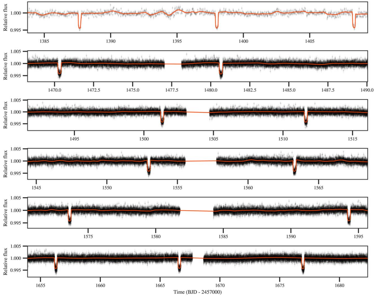
Figure 1. TOI-481 light curves of the six TESS sectors used in our analysis. The top panel presents the TESS Sector 3 data from the full-frame images as black points with error bars obtained with tesseract (see the text), while the rest of the panels show the 2 minute cadence pre-search data conditioning simple aperture photometry light curves for Sectors 6, 7, 9, 10, and 13, respectively. The orange line corresponds to the model obtained in Section 3, which consists of a transit model combined with a Gaussian process that describes the remaining flux variability.
