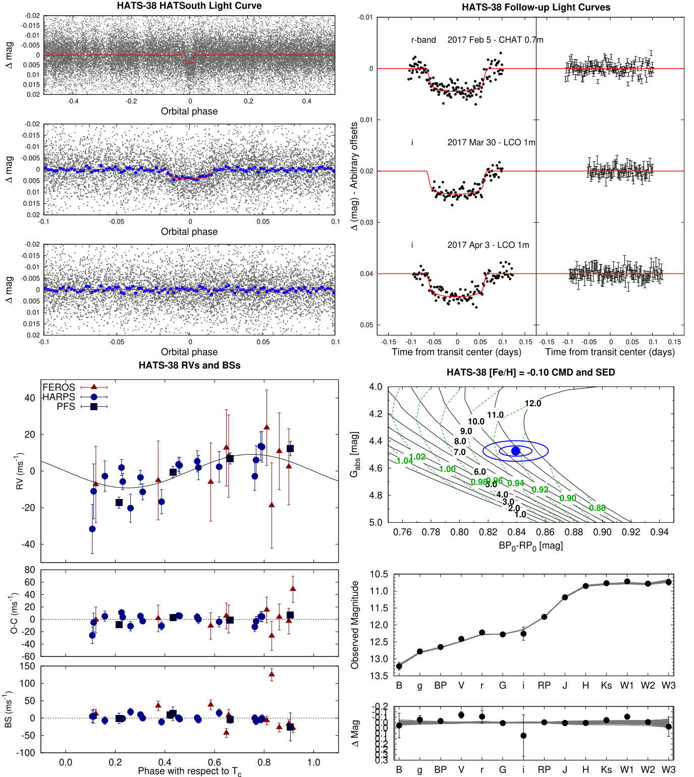
Figure 2. Same as Figure 1. Here we show the observations of HATS-38 when it is modeled as a single star with a transiting planet.
