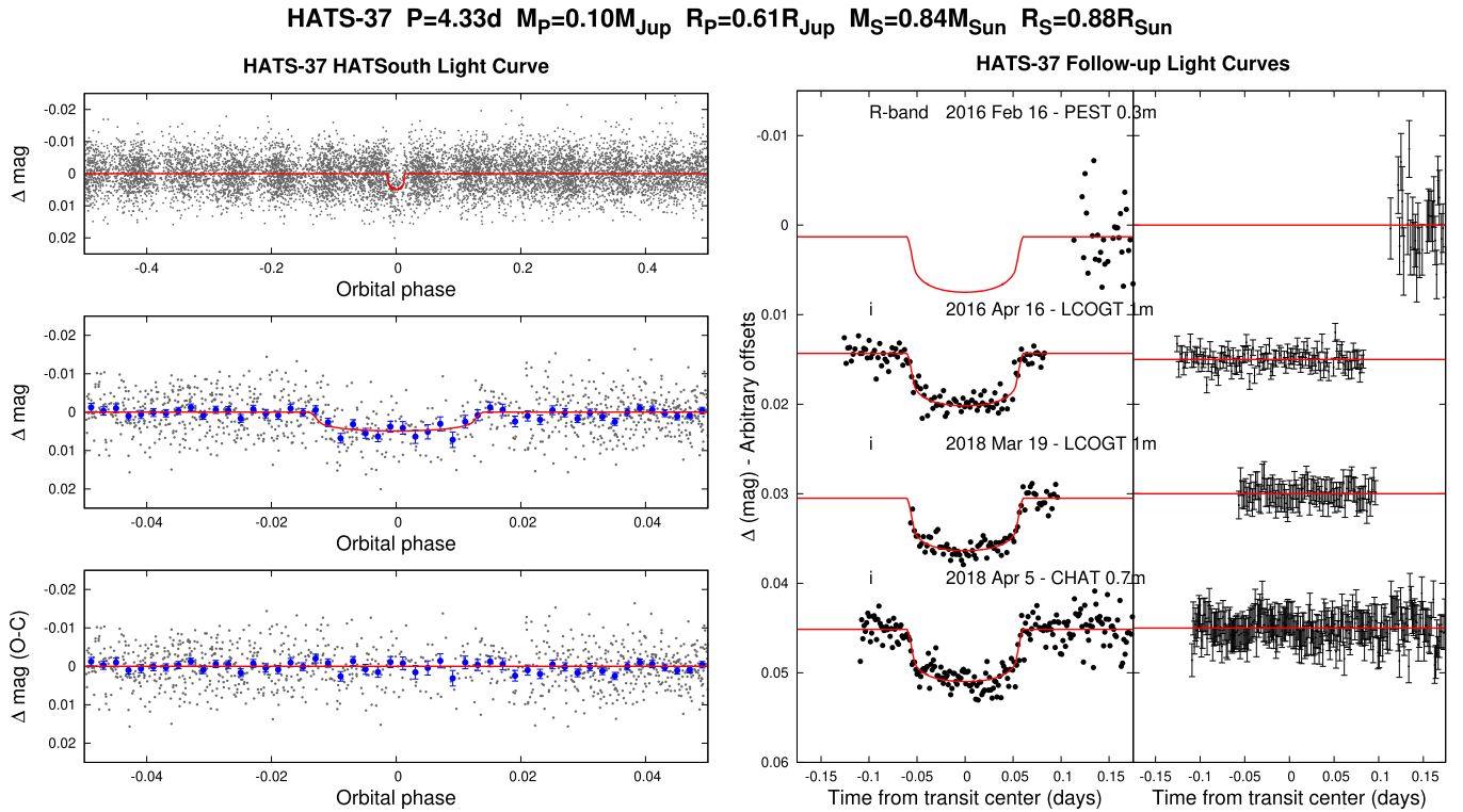
Figure 1. Observations used to confirm the transiting planet system HATS-37. Top left: phase-folded unbinned HATSouth light curve. The top panel shows the full light curve, the middle panel shows the light curve zoomed in on the transit, and the bottom panel shows the residuals from the best-fit model zoomed in on the transit. The solid lines show the model fits to the light curves. The dark filled circles show the light curves binned in phase with a bin size of 0.002. Top right: unbinned follow-up transit light curves corrected for instrumental trends fitted simultaneously with the transit model, which is overplotted. The dates, filters, and instruments used are indicated. The residuals are shown on the right side in the same order as the original light curves. The error bars represent the photon and background shot noise, plus the readout noise. Note that these uncertainties are scaled up in the fitting procedure to achieve a reduced \chi^2 of unity, but the uncertainties shown in the plot have not been scaled. Bottom left: high-precision RVs phased with respect to the midtransit time. The instruments used are labeled in the plot. The top panel shows the phased measurements together with the best-fit model. The center-of-mass velocity has been subtracted. Both the observations and the model have also had a linear trend in time subtracted (Figure 5). In this case the model has not been corrected for dilution from the unresolved stellar component HATS-37B. We find that the dilution corrected orbit has a semi-amplitude that is \sim 20\% larger than what is shown here. The second panel shows the velocity O - C residuals. The error bars include the estimated jitter. The third panel shows the bisector spans. Bottom right: color-magnitude diagram (CMD) and spectral energy distribution (SED). The top panel shows the absolute G magnitude vs. the dereddened BP - RP color compared to theoretical isochrones (black lines) and stellar evolution tracks (green lines) from the PARSEC models interpolated at the best-estimate value for the metallicity of the host. The age of each isochrone is listed in black in gigayears, while the mass of each evolution track is listed in green in solar mass units. The filled blue circles show the measured reddening- and distance-corrected values from Gaia DR2, while the blue lines indicate the 1\sigma and 2\sigma confidence regions, including the estimated systematic errors in the photometry. Here we model the system as a binary star with a planet transiting one component. The 1\sigma posterior distributions for the primary star HATS-37A and secondary star HATS-37B are shown as red ellipses. The gray ellipse shows the 1\sigma posterior distribution for the combined photometry of the system. The inset shows a zoomed-in view around the primary star and the combined photometry. The middle panel shows the SED as measured via broadband photometry through the listed filters. Here we plot the observed magnitudes with mass 0.84 M_{\odot} , and a secondary star with mass 0.65 M_{\odot} . The second mode consists of a primary star with mass 0.88 M_{\odot} , and a fainter secondary star with mass 0.48 M_{\odot} . The first mode is \sim 35 times more likely based on its representation in the posterior distribution. The model makes use of the predicted absolute magnitudes in each bandpass from the PARSEC isochrones, the distance to the system (constrained largely via Gaia DR2) and extinction (constrained from the SED with a prior coming from the MWDUST 3D Galactic extinction model). The bottom panel shows the O - C residuals from the best-fit model SED.
