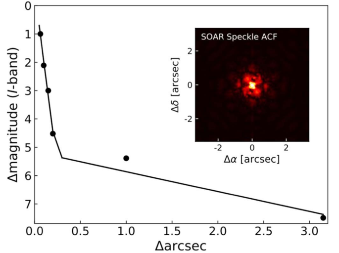
Figure 4. 5\sigma sensitivity limits and auto-correlation functions of the SOAR speckle observations of TOI-569. The black circles are measured data points, and the lines are fits in two different separation regimes. In general, the sensitivity of speckle imaging to companions rises sharply from the diffraction limit to a “knee” at a separation of 0''.15 – 0''.2 , where it then continues to slowly increase out to 1''.5 , beyond which the speckle patterns begin to become de-correlated. No nearby contaminating sources are detected within 3'' .
