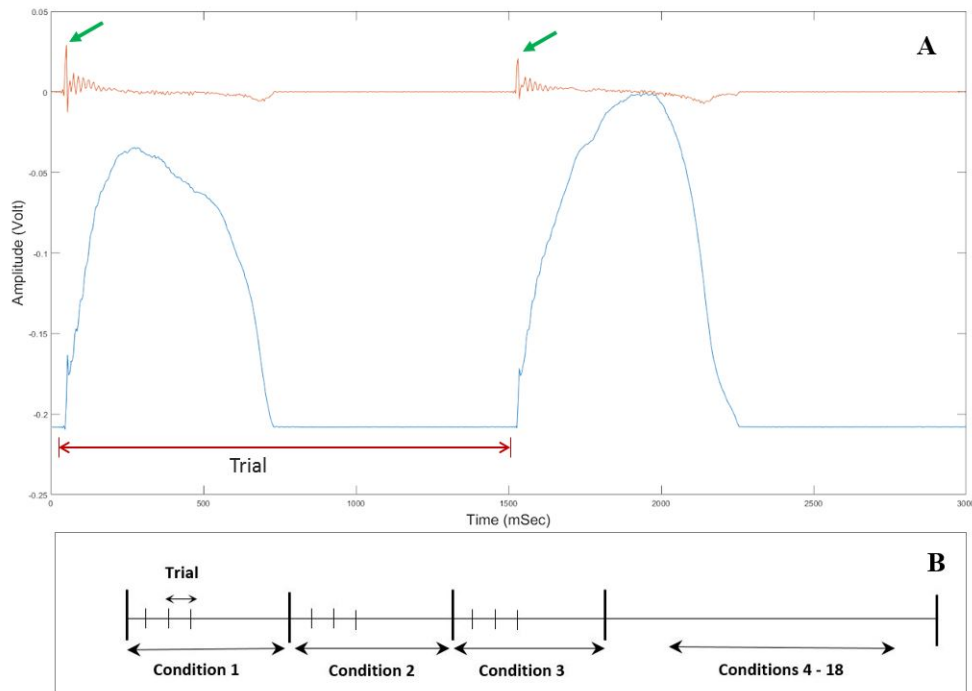
Figure 7. A) The normal force profile, in blue, and the result of applying a first order derivative filter in red. The green arrows show the local peaks that mark the beginning and end of each trial. B) An illustration showing the 18 conditions, and the trials within each condition.
