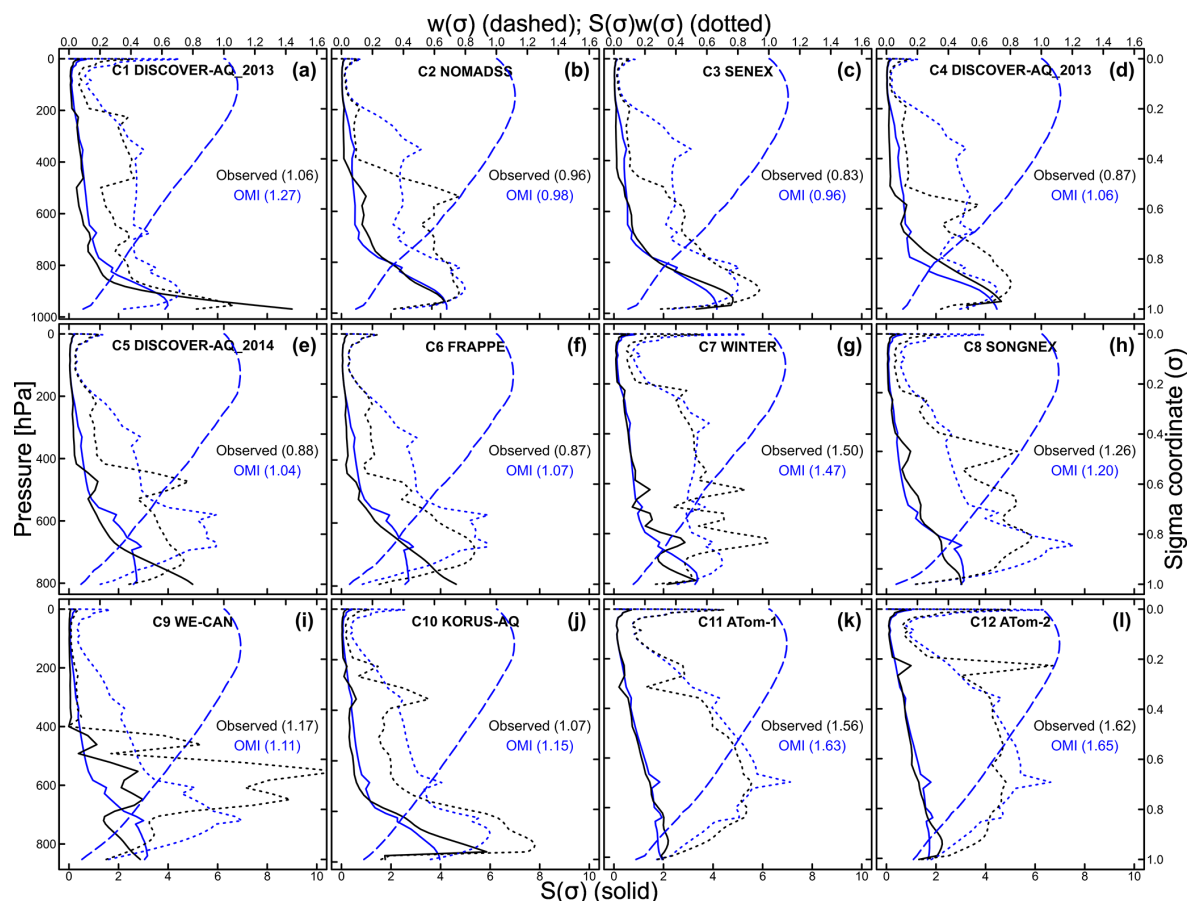
Figure 5. Air mass factor (AMF) components over the 12 aircraft campaigns. Each panel shows mean scattering weights ( w ; dashed blue line) and shape factors ( S ; solid blue line) from the OMI SAO HCHO product averaged over the corresponding grids sampled by the aircraft (marked with open circles in Figs. 4 and S1–S11) during the campaign period (defined in Table 1), as well as the product of the two (dotted blue line) from which mean AMF is derived by vertical integration using Eq. (4). Each panel also shows observed HCHO shape factors (black solid) from the mean HCHO profile in Fig. 3. We use mean HCHO profiles from ATom-1 and ATom-2 (Fig. 3) to fill observations above 6 km. Also shown is the product (dotted black line) of mean OMI scattering weights (dashed blue line) and observed HCHO shape factor (black solid). Mean AMF values are given in the legend computed using OMI (blue) and observed (black) shape factors.
