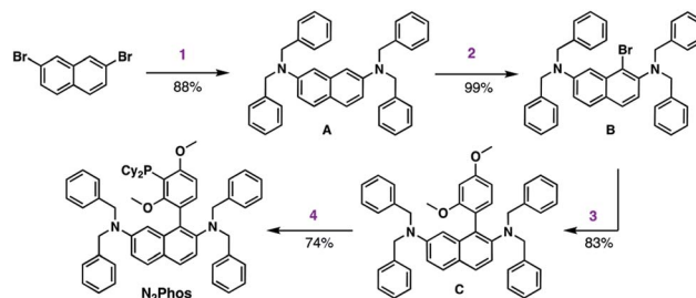
Scheme 2 Synthesis of N 2 Phos. Step 1. 2,7-dibromonaphthalene, Pd-PEPPSI-iPent (2 mol%), dibenzylamine, KO- t -Bu, in toluene at 80 °C. Step 2. A, NBS, in DMF at 0 °C to rt. Step 3. B, 2,4-dimethoxyphenylboronic acid, Pd(OAc) 2 (2 mol%), BI-DIME, K 3 PO 4 ·H 2 O, dioxane, 80 °C. Step 4. C, n -BuLi, THF, 0 °C; then Cy 2 PCL, 0 °C to rt.
