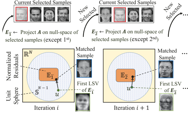
Figure 3: Two consecutive iterations of the SP algorithm. In each iteration the residual matrix, E_k , is computed. The first LSV of the residual matrix, u , is a vector on \mathbb{S}^{N-1} . The most aligned column of E_k with u is selected at each iteration and it is replaced for the next iteration. Please note that E_k \subset \mathbb{S}^{N-1} \subset \mathbb{R}^N in the Venn diagrams.
