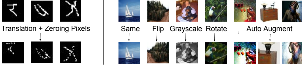
Figure 2: Augmentation techniques on Omniglot (left) and Mini-Imagenet (right). Top row: Original images in training data. Bottom: augmented images for the validation set, transformed with an augmentation function \mathcal{A} . Auto Augment [8] applies augmentations from a learned policy based on combinations of translation, rotation, or shearing.
