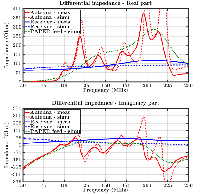
Figure 4. Differential input impedance of the RF receiver and of the antenna, from measurements ("meas") and simulations ("simu").
