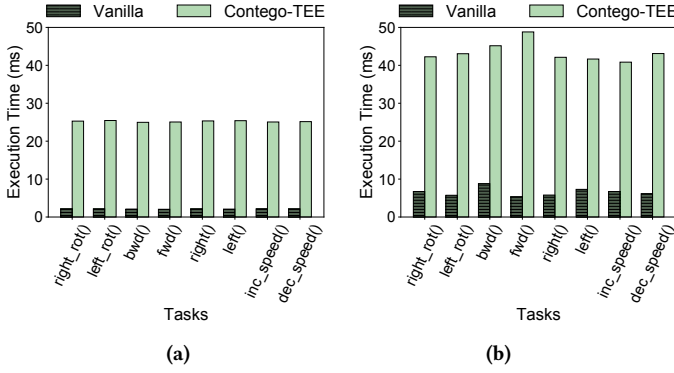
Figure 5: Runtime of rover control tasks with and without Contego-TEE: (a) for 99-th percentile and (b) worst-case. Contego-TEE increases the execution time by upto 43.47 ms (worst-case) and 23.31 ms (99th-percentile).
