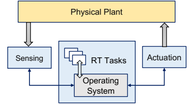
Figure 2: Schematic of a RT control system.
