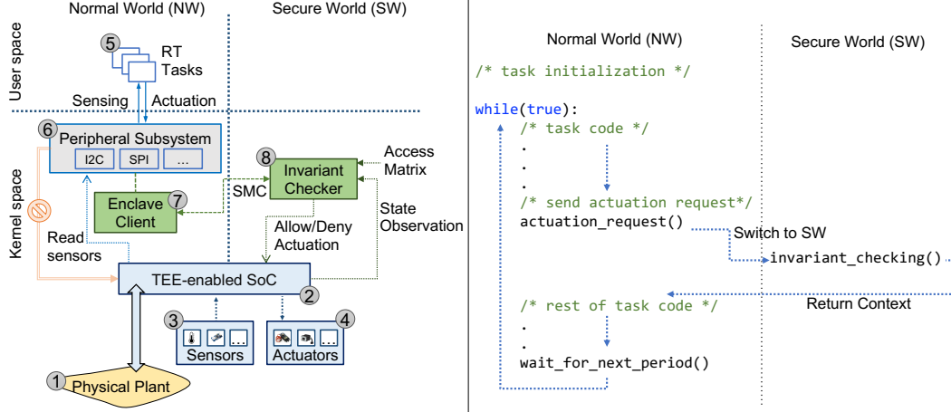
Figure 3: Overview of Contego-TEE system design (left) and high-level control flow of RT tasks in Contego-TEE (right).
