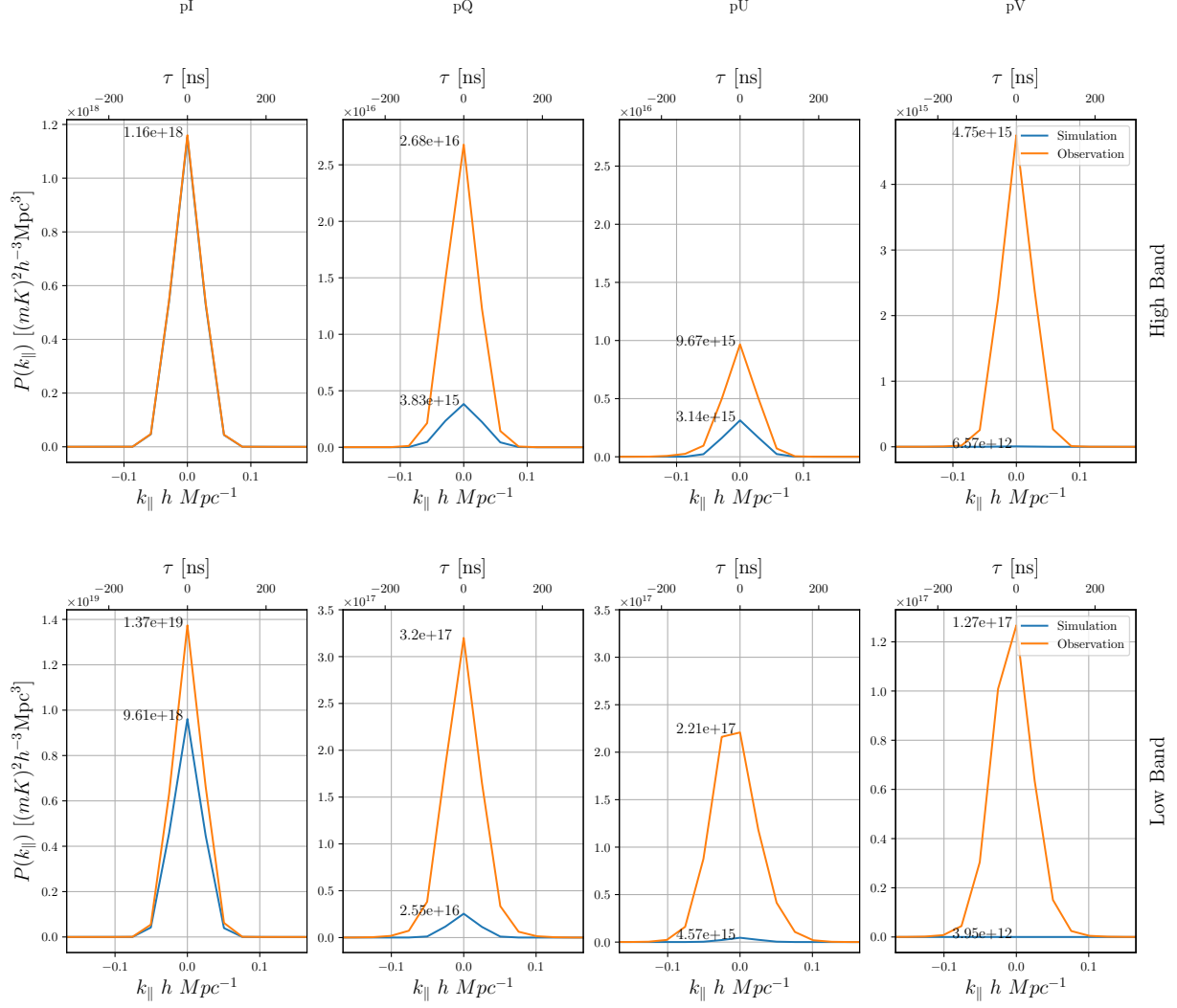
Figure 11. A zoom in on Figure 10 showing just the k_{\parallel} values near the wedge, and with a linear scale in P(k_{\parallel}) . Note that the scale changes for each Stokes for each parameter, except that Q and U are set to have the same scale in each row.
