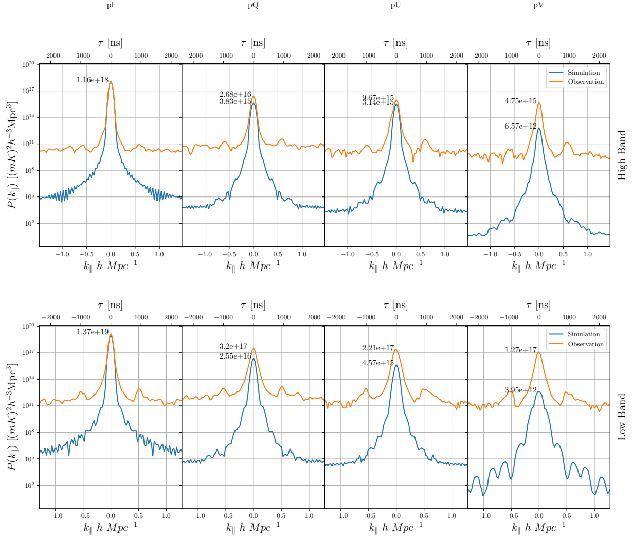
Figure 10. Simulated and observed power as a function of k_{\parallel} for the shortest baseline (14.6 m). Left to right : pseudo-Stokes I, Q, U and V; above : the high band; below : the low band. The simulations were noiseless and used an unpolarized sky model. The agreement with Stokes I is excellent in the high band, and consistent with an absolute calibration accuracy of \sim 20\% for the low band. The agreement between the simulations and the data for the other pseudo-Stokes parameters is poor, as discussed in the text, likely due to a combination of calibration errors, particularly for Stokes V, and actual polarized emission.
