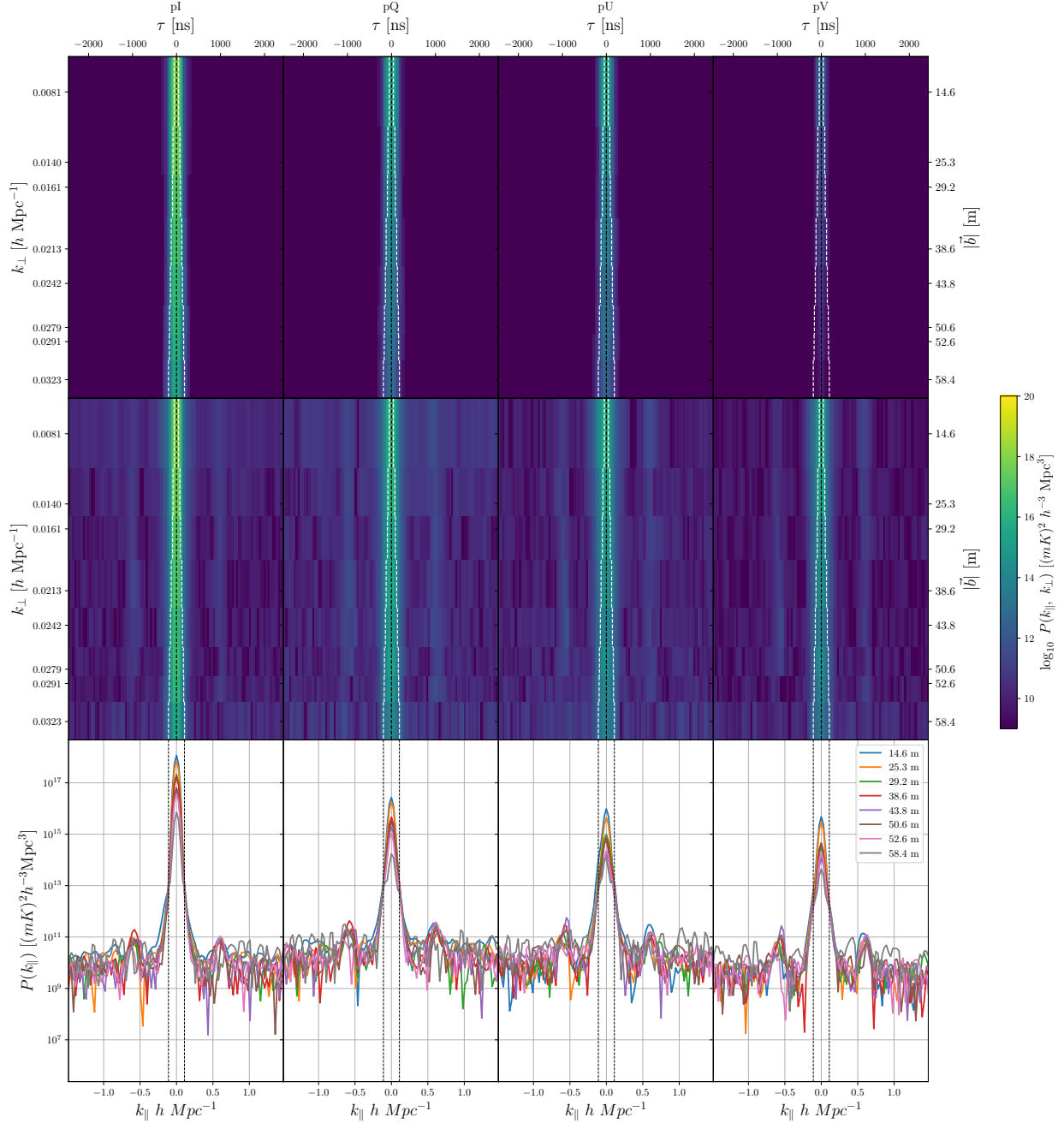
Figure 8. Results from the high-band (157–167 MHz). Top: Simulated power spectra in Stokes I, Q, U and V, following the formalism in Section 2. No polarized sky model was used, so power in Stokes Q, U and V is only due to the direction-dependent beam leakage from Stokes I. No instrumental noise was included in the simulation. Middle: Eight-day average power spectra from data. Bottom: The same data as shown in the middle panel, but with each baseline length overlaid on one another to allow shared features to be more easily identified. For the top and middle plots, white dotted lines indicate the boundary of the pitchfork and the EoR window for that baseline length. A black dotted line indicates the k_{\parallel} = 0 h/Mpc line. In the bottom panel, dotted lines indicate the boundary of the wedge for the longest baseline only. Delays in nanoseconds are indicated along the top, and the corresponding cosmological k at the mean redshift along the bottom axis.
