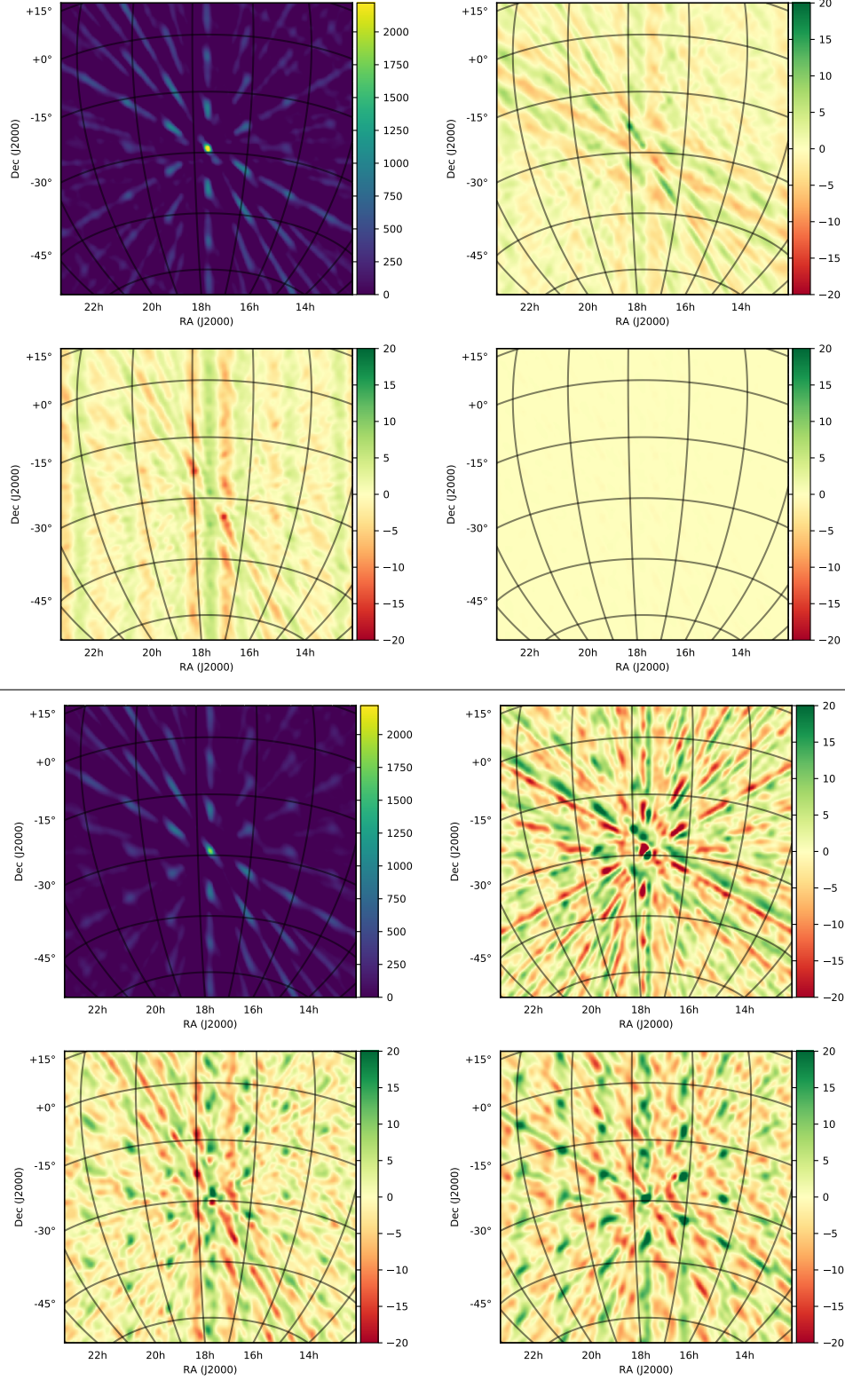
Figure 7. Both sets of panels show multi-frequency synthesis pseudo-Stokes images of I, Q, U and V visibilities ( top left, top right, lower left, lower right ) for the Galactic Center (our calibration source) at transit. Note the field-of-view shown is about 60^\circ across. A Briggs-weighting with robustness 0 was used when gridding into the image plane. No deconvolution was performed. The colorbar is in units of Jy/Beam. A separate color scale is used for Stokes I for suitable dynamic range in the polarized fluxes; note that the color scales differ by a factor of 100. Above: Simulation, where only a Stokes I sky was used; any polarized power is due to direction-dependent polarization leakage (see Section 2.1). Below: Multi-frequency synthesis pseudo-Stokes images formed from observed visibilities on JD 2457548.
