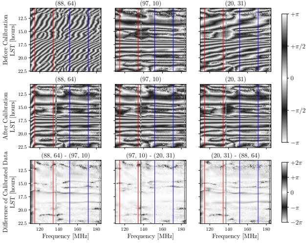
Figure 6. The effect of calibration on the phases of visibilities from three redundantly-spaced 14.7 m baselines; nn polarization. The antenna numbers refer to those given in Figure 3. The color scale is cyclic; black is \pm\pi/2 and white is 0 and \pm\pi . The extent of the low band is indicated with red lines and the high band with blue. Top row : before calibration; Middle row : after calibration; Bottom row : the three pairs of differences of the calibrated phases. Note that the agreement between baselines is excellent near the Galactic Center but shows significant differences at some other times.
