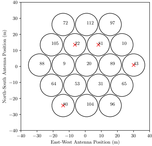
Figure 3. The configuration of the HERA-19 array. The perimeter of each dish is shown as a circle. A red “X” marks antennas that were identified during preprocessing and calibration as malfunctioning and were excluded from further analysis.
