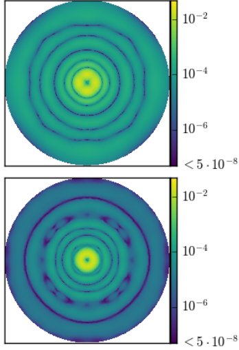
Figure 2. The magnitude of the linear polarization leakage beam given by \mathcal{M}_p = \sqrt{\mathcal{M}_{IQ}^2 + \mathcal{M}_{IU}^2} , or the middle two entries of the top row of Figure 1, at 120 MHz and 160 MHz (above and below, respectively).
