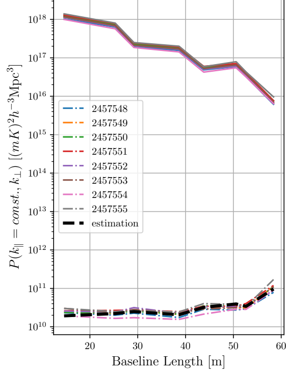
Figure 12. High band power as a function of baseline length for k_{\parallel} = 0 h/Mpc (solid lines) and an average value over the white noise ( |k_{\parallel}| > 1 h/Mpc; dot-dashed lines) for pseudo-Stokes I on each JD of observation. The black dashed line represents estimated power spectrum noise given a system temperature of 2400 K. A very similar relationship obtains for the low band (not shown), but with a higher system temperature of 7000 K. Note that the increase of the noise level with baseline length is correctly modeled, as the compact array has a decreasing number of baselines which are averaged together in a given (k_{\parallel}, k_{\perp}) bin.
