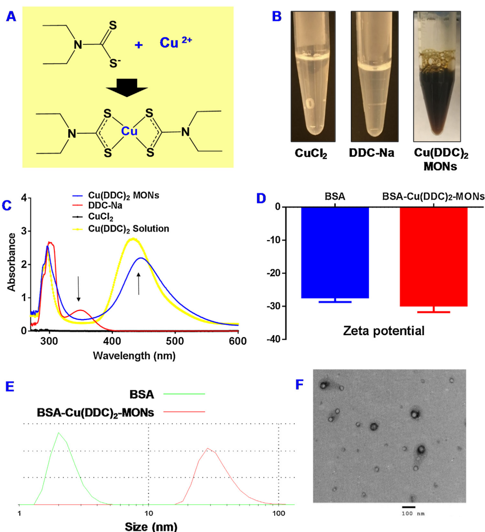
Fig. 1. Characterization of BSA \text{Cu(DDC)}_2 MONs. (A) Schematic illustration to show the \text{Cu(DDC)}_2 complex formation. (B) Photos of \text{Cu(DDC)}_2 MONs, DDC-Na and \text{CuCl}_2 . (C) The spectrum of \text{Cu(DDC)}_2 solution, DDC-Na, \text{CuCl}_2 , and \text{Cu(DDC)}_2 MONs. (D) Zeta potential. (E) Particle Size. (F) TEM of BSA \text{Cu(DDC)}_2 MONs.
