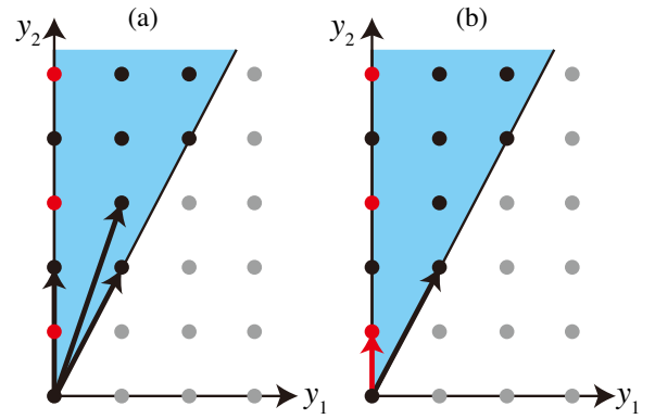
FIG. 3. (a) EFPs in SG 199 ( I2_13 ). The shaded area represents the cone Y , the black points represent the trivial points in \tilde{Y} , the red points represent the EFPs, and the grey points correspond to unphysical symmetry data. The three bold vectors (0,2)^T , (1,2)^T , (1,3)^T are the generators of trivial points. (b) The Hilbert bases of \tilde{Y} . The two bold vectors, i.e., (0,1)^T , (1,2)^T , generate all the points in \tilde{Y} . Here, (0,1)^T is nontrivial and corresponds to a fragile root, and (1,2)^T is trivial and corresponds to an EBR.
