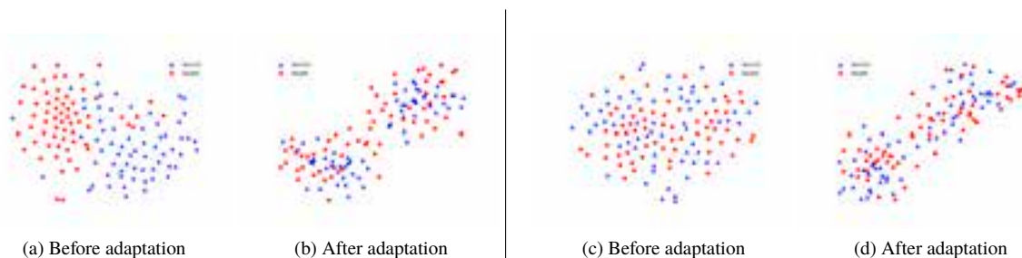
Figure 3. Two dimensional representation of source (blue) and target (red) using the VGG-19-SL representation of the images (before adaptation), and the DANN-SL-TU transformed representation of the images (after adaptation), for two pairs of disasters. The pair on the left consists of two dissimilar disasters, Ecuador Earthquake (source, blue) and Ruby Typhoon (target, red). The pair on the right consists of two similar disasters, Ecuador Earthquake (source, blue) and Nepal Earthquake (target, red). The two representations are reduced to 2 dimensions using the t-SNE (Van Der Maaten 2014) technique.
