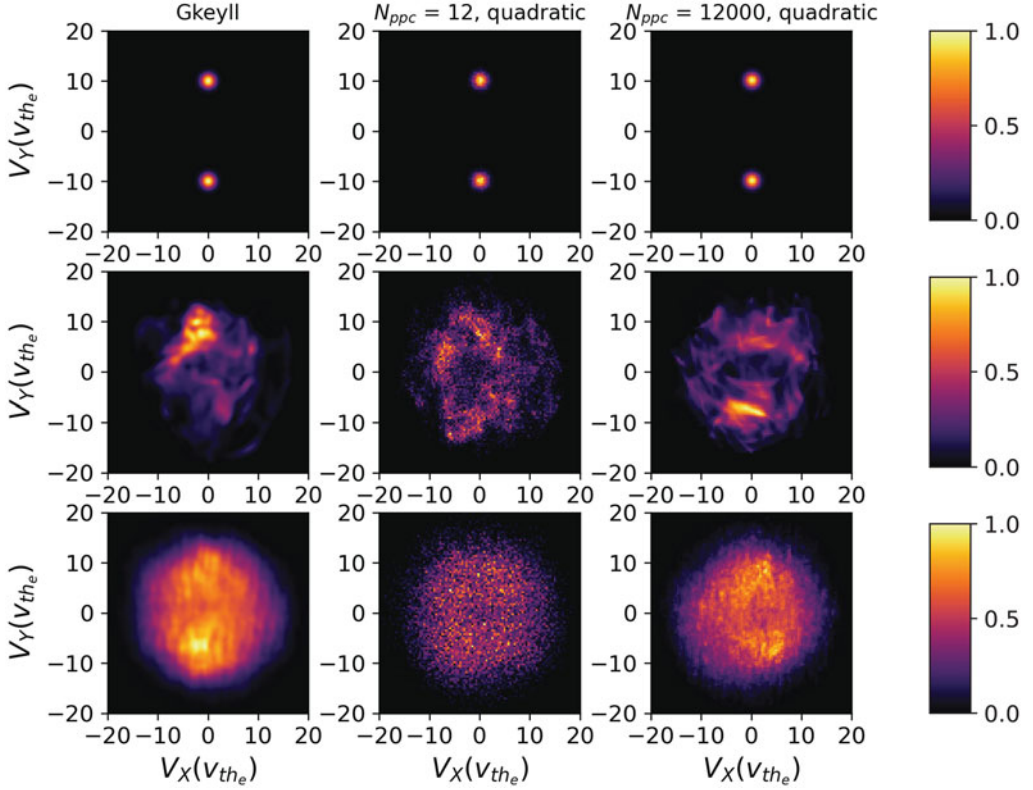
FIGURE 3. The same evolution of the electron distribution function shown in figure 2 from Gkeyll (left column) and N_{\text{ppc}} = 12 and N_{\text{ppc}} = 12\,000 , quadratic spline, p3d (middle and right column) simulations, but now in v_x - v_y . The rows show the evolution of the distribution function in time, t = 0\omega_{\text{pe}}^{-1} (top row), the peak of the magnetic field energy, t = 45\omega_{\text{pe}}^{-1} for the Gkeyll simulation and t = 35\omega_{\text{pe}}^{-1} for the p3d simulations (middle row) and the end of the simulation t = 250\omega_{\text{pe}}^{-1} (bottom row). These distribution function cuts are generated by integrating over a narrow slice of the interior of L_x and all of y . As in figure 2, we integrate the Gkeyll simulation over the middle two grid cells, \Delta x = 0.1d_e , and sample particles from the corresponding extent in the p3d simulations. In addition, to generate the velocity space representation in v_x and v_y of the p3d simulations, the particles are binned into 101 equally space bins from -20v_{\text{the}} to 20v_{\text{the}} for both velocity dimensions. Again, the phase space resolution at the beginning of the simulation is acceptable, even with only N_{\text{ppc}} = 12 , because we can sample particles efficiently for the cold distribution. However, because the unstable oblique modes efficiently convert this free energy into electromagnetic energy and then back into electron thermal energy, the final electron distribution fills a much larger volume of phase space and the effective phase space resolution has plummeted by the end of the simulation.
