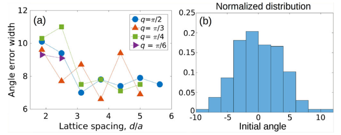
FIG. 8. Error in initial orientation. (a) The error is quantified by 0.5(\text{maximum-minimum}) of the initial angles in any given run. This measure of the width in release angle is plotted here as a function of lattice spacing for qd = \pi/2, \pi/3, \pi/4 , and \pi/6 . (b) A combined distribution of initial angles of several experimental runs for a fixed qd = \pi/2 and d = 3.75a .
