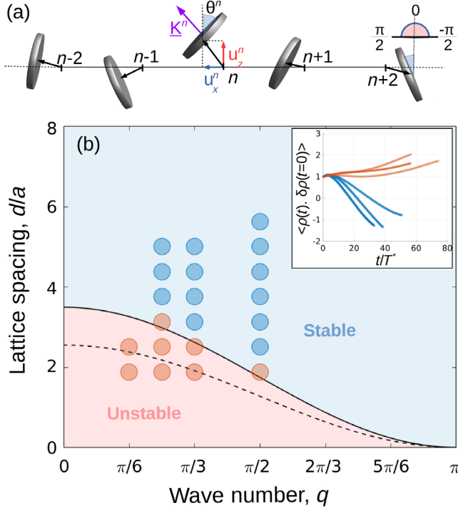
FIG. 4. Phase diagram. (a) A schematic of the array of disks showing spatial perturbations ( u_x^n , u_z^n ) and orientation perturbation \theta^n of the n th disk which interacts hydrodynamically with the neighbors n-i , i = 1, 2, \dots . For prolate spheroids the orientation vector \mathbf{K}^n is rotated by \pi/2 from the one shown. (b) The phase diagram with the stable regime shown in blue and unstable regime in red. The experimental data points (circles) are colored blue or red by measuring whether the density autocorrelation grows or decays, which is shown in the inset of (b), for some representative stable (blue) and unstable (red) points in the q-d plane, where timescale T^* = \mu d^2/F . The phase boundary predicted by the linear theory with nearest-neighbor interaction is shown for oblate spheroids with eccentricity approximating the experimental thickness, e = 0.9922 (solid line) and spheroid of zero thickness e = 1 (dashed line).
