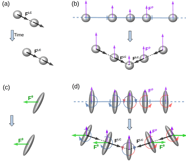
FIG. 1. Schematic of competing mechanisms. (a) F^{LC} acts on the pair along the line joining their centers leading to horizontal drift. (b) Clumping of array of spheres results from the line-of-centers force F^{LC} , acting along with reduced drag force F^D . (c) A spheroid drifts laterally as it falls when it is oriented obliquely with respect to gravity. (d) Lateral drift F^\theta competing with the clumping induced by F^{LC} and F^D .
