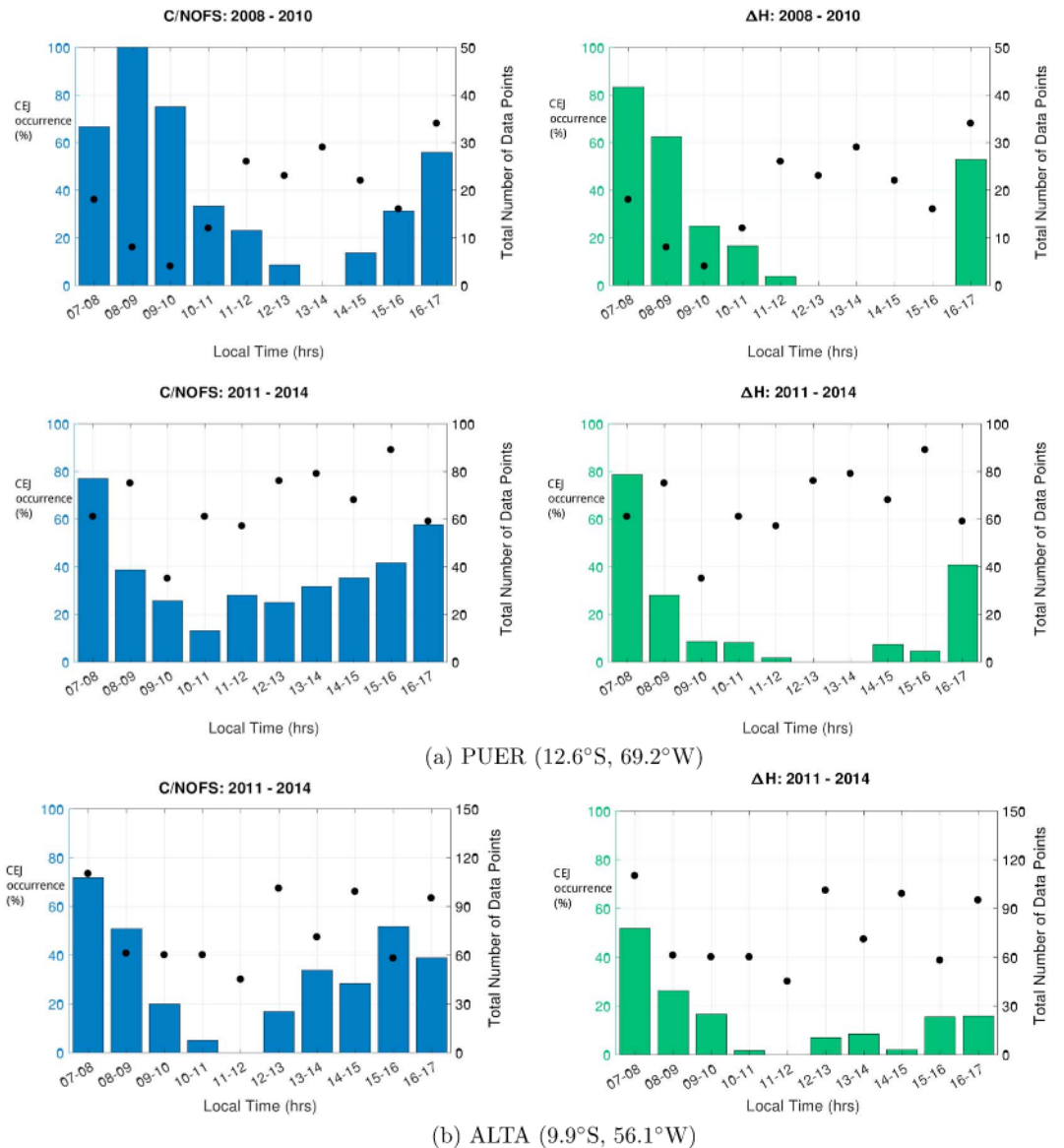
Figure 4. Local time observations of CEJ occurrences as observed from C/NOFS satellite and ground-based magnetometer data, separately during 2008–2010 and 2011–2014 over (a) PUER (12.6°S, 69.2°W) and (b) ALTA (9.9°S, 56.1°W), within the American sector. CEJ = counter electrojet; C/NOFS = Communications and Navigation Outage Forecasting System.
