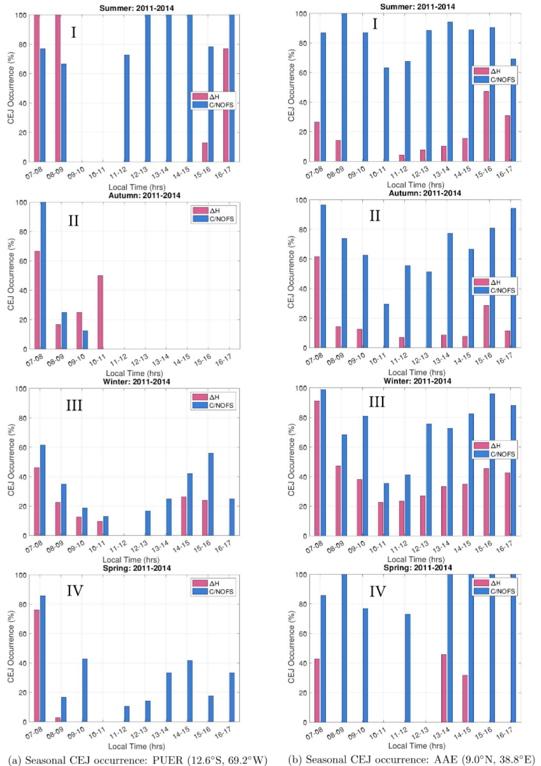
Figure 7. Seasonal occurrence of CEJ (expressed as a percentage) as observed by C/NOFS satellite (blue) and ground-based magnetometers (dark pink) over the American and African sectors during 2011–2014. CEJ = counter electrojet; C/NOFS = Communications and Navigation Outage Forecasting System.
