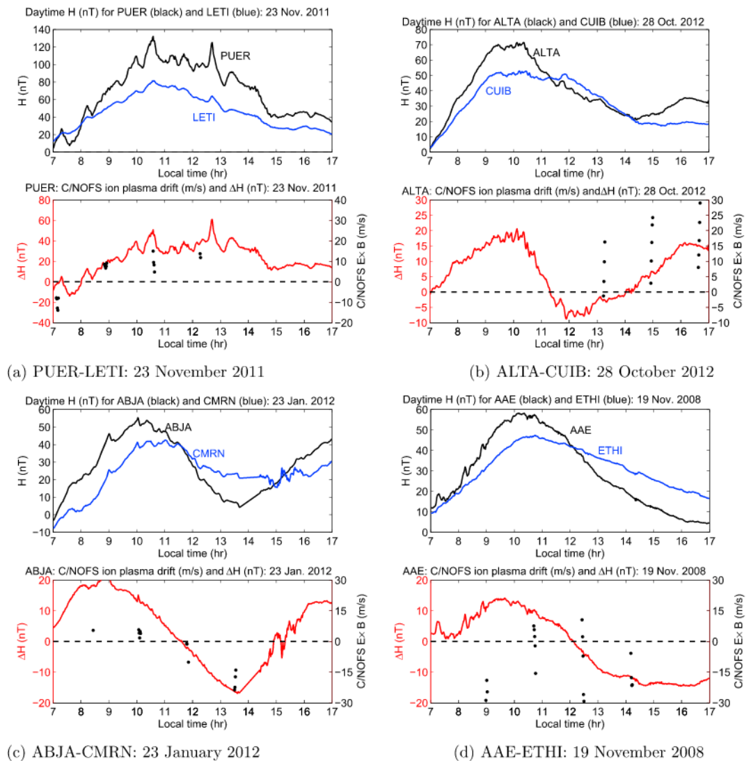
Figure 2. Examples of horizontal component of the geomagnetic field with derived equatorial electrojet changes and available C/NOFS vertical ion plasma drift ( E \times B drift, plotted as black dots) for longitude sectors of (a) 69°W (23 November 2011), (b) 56°W (28 October 2012), (c) 9°E (23 January 2012), and (d) 39°E (19 November 2008), respectively. C/NOFS = Communications and Navigation Outage Forecasting System.
