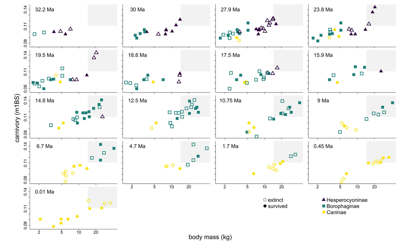
Fig. 2 Ecomorphology of extinct and survived canid species over 17 time slices. Gray boxes designate the large-hypercarnivore niche. Only the end-Pleistocene extinction, at 0.01 Ma, shows a significant difference in body mass and carnivory between extinct and survived.
