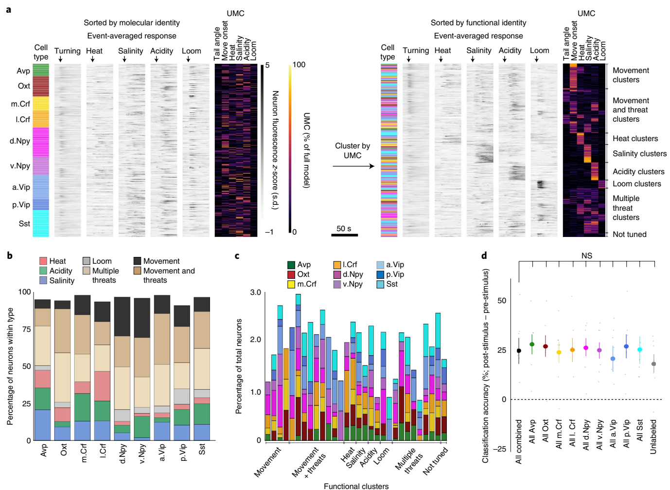
Fig. 3 | Behavior-specific neural ensembles span multiple neuropeptidergic hypothalamic populations. a , All identified peptidergic neurons recorded ( N=452 peptidergic neurons from 28,211 total recorded cells in 7 fish), with the cell population denoted by color, event onset-averaged responses indicated by gray intensity and UMC values from the linear model fit displayed as a heatmap (percentage of full model). Left: neurons were sorted by molecular and anatomical identity. Right: after clustering UMC values, the same neurons were sorted by functional identity (cluster identity written on the right). b , Cluster identities for each molecular and anatomical cell population examined ( N=7 fish, number of neurons in each cell population (from left to right) = 33, 53, 37, 44, 75, 48, 63, 28 and 71). ‘Movement’ encompasses ‘tail angle’ and ‘move onset’ clusters. The ‘not tuned’ cluster is not displayed. c , The cell populations within each functional cluster, plotted as percentage of all neurons in the cluster (including unlabeled neurons). Details of each functional cluster is presented in Extended Data Fig. 6. d , Differences in the mean threat classifier accuracy between the time after threat onset compared with before threat onset across cell populations ( N=7 fish). Data shown for all peptidergic neurons together and with neurons from individual cell classes removed. Data are shown as the mean \pm s.e.m., with points representing individual fish. All comparisons are two-tailed t -tests with the ‘All combined’ group (all recorded peptidergic neurons), Benjamini-Hochberg false discovery rate correction for multiple comparisons. NS, not significant, all P>0.3 . See Supplementary Table 2 for test statistics.
