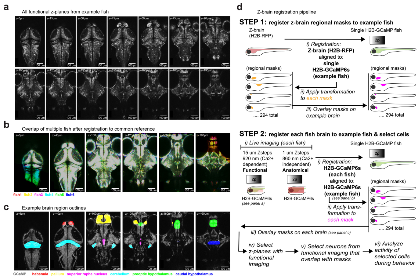
Extended Data Fig. 2 | Coverage, registration, and anatomical segregation of brain-wide imaging data. a , All z-planes functionally imaged in a single Tg(elavl3:H2B-GCaMP6s) fish - 14 z-planes, 15 μm separation, 2 volumes/second. All N = 8 fish were imaged with the same x/y/z-sampling. b , Example z-planes from N = 6 fish, after registration to a common volume. Fish were registered to a common 'bridge' brain; the standard Tg(elavl3:H2B-RFP) brain from the Z-Brain atlas (along with atlas masks) were registered to this bridge brain, to allow for anatomical region analysis. c , Example z-planes from a single fish, with a subset of overlaid anatomical regions from the registered Z-Brain atlas. The same regions were aligned to each of the N = 8 fish. d , Step-by-step protocol for registering each recorded brain to a common volume, and assigning recorded neurons to brain regions in the Z-brain atlas.
