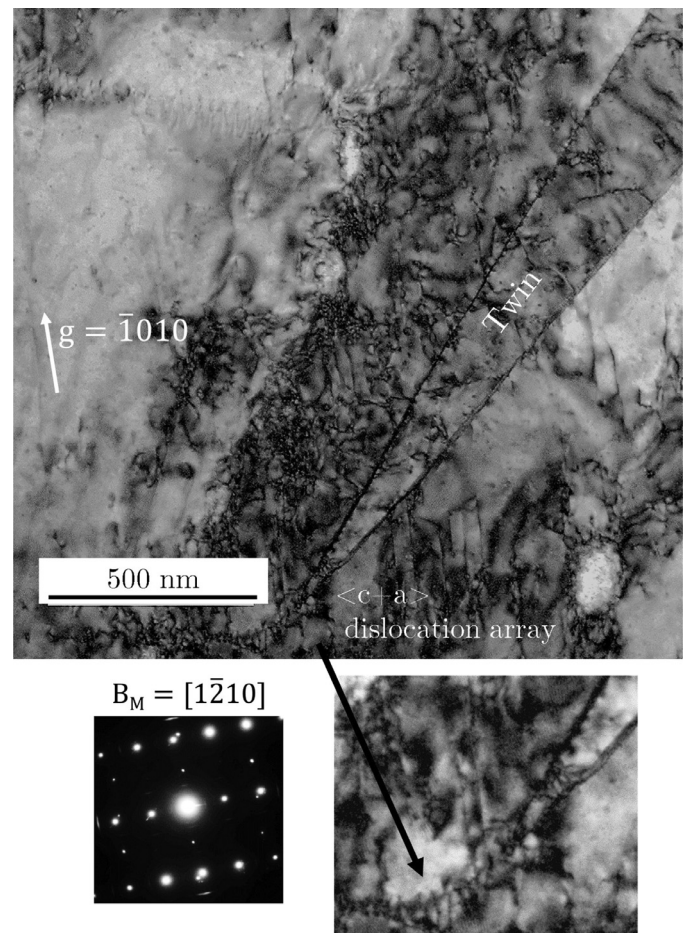
Fig. 8. (a) TEM image of another tensile twin tip which has stopped propagating inside grain-3 of the deformed alloy. The matrix is oriented along the [1210] direction. The experimental SAED pattern shows the spots corresponding to twin as well as the matrix and is consistent with the tensile twinning. The black arrow points a \langle c+a \rangle dislocation array, which is associated with the twin tip, and is similar to the case of twin tip described in Fig. 3.
