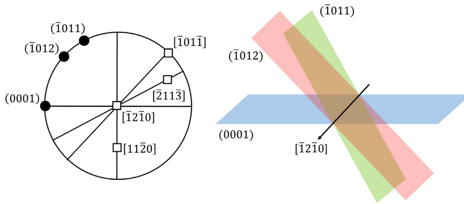
Fig. 7. Standard hcp Mg stereographic projection showing the relation between \{1012\} twinning plane and the glide planes of \langle a \rangle and \langle c+a \rangle dislocations observed in this study. The corresponding Burgers vectors of twinning partials and matrix dislocations are also displayed on the projection. It is clear that the twinning plane and glide planes of matrix dislocations share [1210] as a common line of intersection as illustrated in the schematic.
