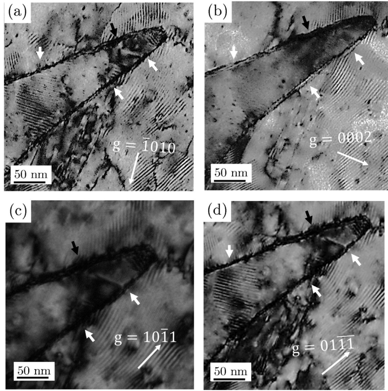
Fig. 5. Magnified view of the tensile twin tip which has terminated inside grain-1. The images were obtained under two different zone axes: (a), (b), (c) [1\bar{1}2\bar{3}] and (d) [1\bar{2}1\bar{3}] and for various operating reflections as described in Fig. 4. The black and white colored short arrows point the changes in diffraction contrast at some specific regions along the twin boundary, and for the operating reflections displayed on the micrographs.
