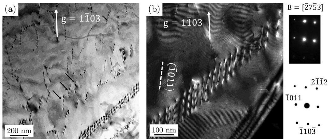
Fig. 2. TEM images of the same glissile pyramidal-I \langle c+a \rangle slip dislocations shown in Fig. 1, however, for the [2\bar{7}53] orientation and for g = 1\bar{1}03 reflection of the matrix (a). Weak beam dark field image of the intragranular sub-boundary showing the projections of dislocations parallel to the trace of (1011) pyramidal-I plane (b).
