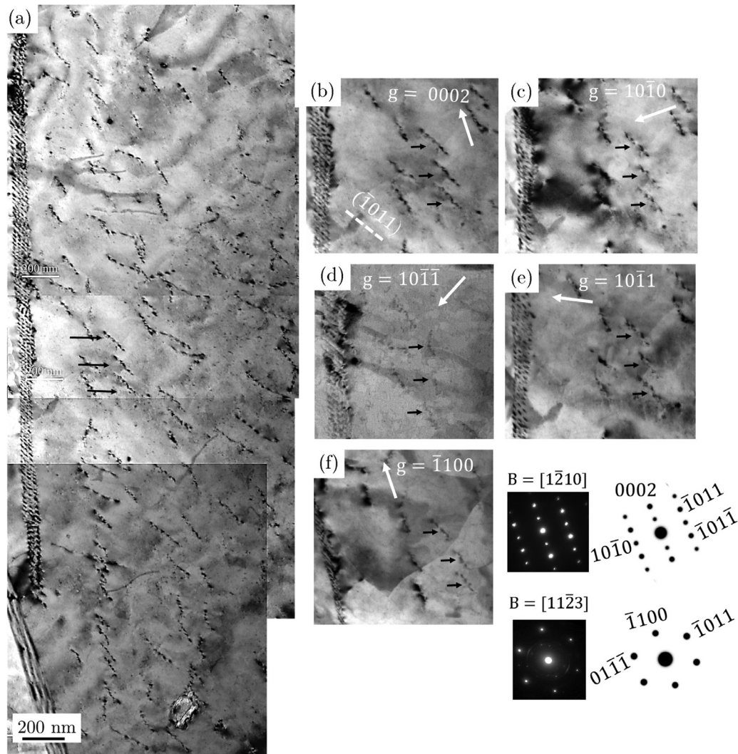
Fig. 1. A bright field TEM micrograph of the deformed microstructure obtained from a twin-free grain (i.e. grain-2). The microstructure consists of slip dislocations and an intragranular sub-boundary associated with an array of dislocations (a). The images (b)-(f) were acquired under two-beam bright field diffracting conditions using various operating reflections as mentioned on each micrograph, and for the [1\bar{2}10] and [11\bar{2}3] orientations of grain-2. The corresponding SAED patterns are also provided in the image along with the simulated patterns. The black colored arrows pointing three dislocations indicate the variation in dislocation contrast for different operating reflections. The white colored dashed line represents the traces of (1011) pyramidal-I plane, which is in an edge-on orientation (b).
