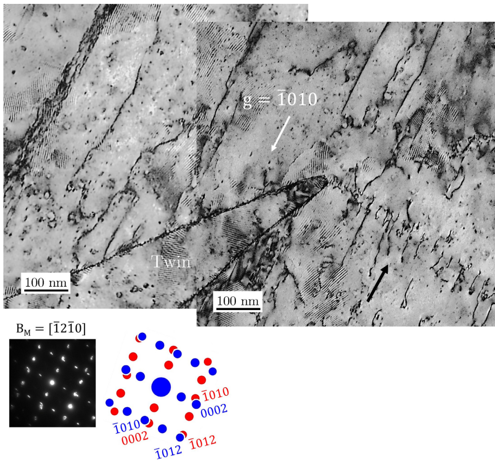
Fig. 3. (a) TEM image of a tensile twin terminating inside the grain-1 of deformed alloy. The grain-1 is oriented along the [\bar{1}2\bar{1}0] direction. The experimental SAED pattern is provided along with the simulated pattern, where blue colored spots represent the matrix and red colored spots represent twin. The black colored arrow on the plane of the micrograph represents a dislocation array, which appears to be connected with the twin tip. (For interpretation of the references to colour in this figure legend, the reader is referred to the web version of this article.)
