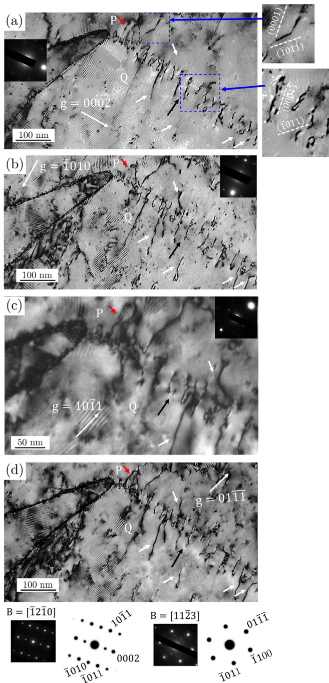
Fig. 4. Two-beam bright-field TEM images of (\bar{1}012) tensile twin terminating inside the grain-1 of the deformed alloy. The images were acquired under (a), (b), (c) [\bar{1}2\bar{1}0] , and (d) [11\bar{2}3] orientations of grain-1, and using various operating reflections. The corresponding SAED patterns are also provided along with the simulated patterns. The white colored dashed lines represent the traces of the basal and (\bar{1}011) pyramidal-I planes (a). The short white colored arrows indicate the basal \langle a \rangle dislocations in the array, while rest of the dislocations in the array are found to be \langle c+a \rangle (indicated by a black arrow).
