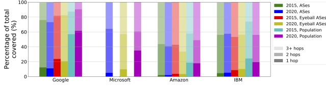
Figure 13: Comparison of path length to reach destination networks from Amazon, Google, IBM, and Microsoft in 2015 and 2020 (number of hops is number of inter-AS links, so one hop indicates direct peering from cloud provider to destination network; Microsoft 2015 traceroute data not available). The path lengths are weighted in three ways: as percent of total networks, as percent of networks hosting users, and as percent of users they host [2]. Path length has remained relatively stable over time, even when weighted by population.
