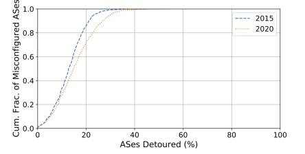
Figure 10: Cumulative fraction of detoured ASes when Google announces routes to all its peers in the 2015 and 2020 Internet. Results show small improvement in resilience, as Google reduced its number of providers and most new peers are small edge ASes.
