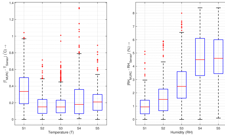
Figure 8. A comparison of the sensor readings with the MURC tower: The data presented here summarizes 10 minutes of hover at the MURC tower altitude (15.2 m) as presented in Figure 7. (S1—P1XQ1 (housing), S2—P1XQ2 (housing), S3—P2XQ2 (housing), S4—P2Nimbus1 (no housing), and S5—P2Nimbus2 (housing)).
