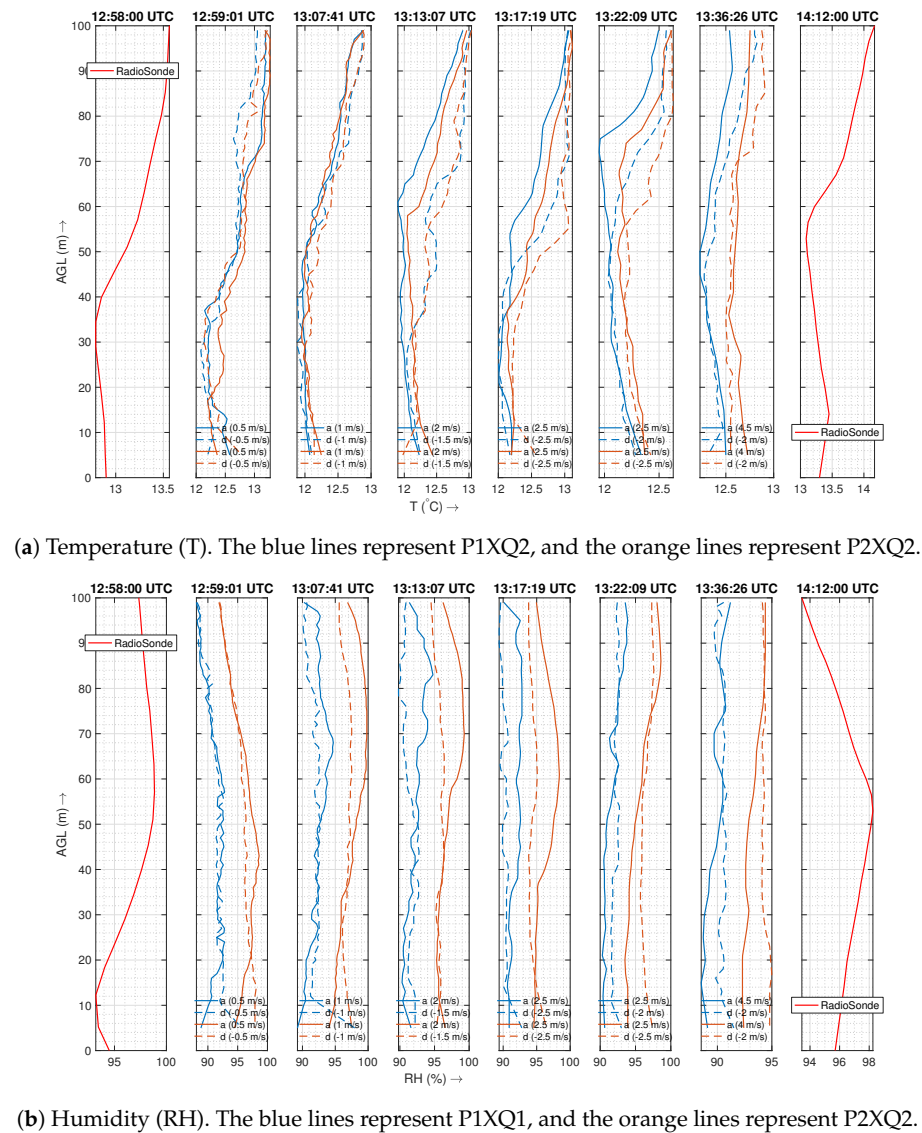
Figure 11. The plot shows two radiosonde flights (filtered and corrected) and six different flights of the UAS (not filtered/corrected) at different speeds in an inversion layer. The surface wind was 2 m/s from 290–308° relative to north and with a partly cloudy sky. The P1XQ2 sensor is upstream, while the P1XQ1 and P2XQ2 sensors are downstream from the UAS with respect to wind.
