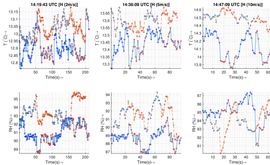
Figure 13. The plot shows three different horizontal “transect” flights at different horizontal (H) speeds at 50 m AGL. The surface wind was 2 m/s from 290–308° relative to the north, and the sky is partly cloudy. The solid line plots indicate data from M600P1, and the dashed lines indicate data from the M600P2. The blue (M600 P1) and light blue (M600 P2) scatter dots indicate transects 1 and 3, while the red (M600 P1) and orange (M600 P2) are transects 2 and 4. Figure 12 shows the direction of air flow inside the housing, the surface wind, and the horizontal transects for each of the transects for both UASs. The data shown here is not filtered/corrected for sensor response characteristics.
