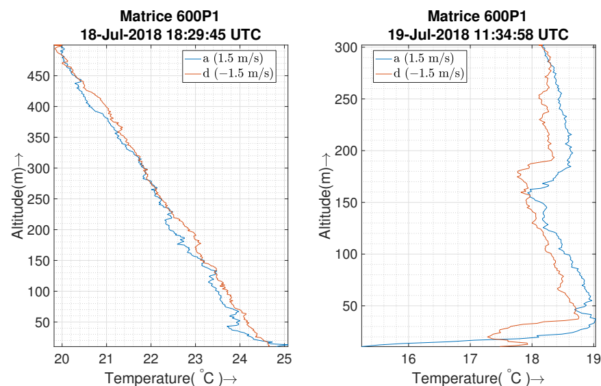
Figure 14. The first subplot shows unfiltered temperature data collected from 10 m–500 m of a well-mixed atmosphere at noon with a ground wind of 1.6 m/s with a 5 m/s gust.
