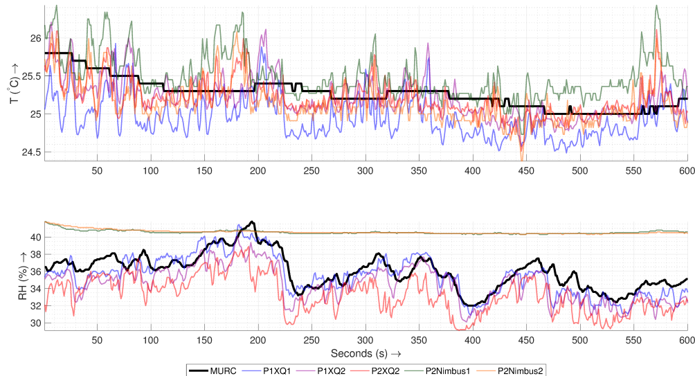
Figure 7. The Temperature (T) and Humidity (RH) time series of the MURC tower and other sensor readings for the 10 min of hover of the UAS at the MURC tower altitude (15.2 m): Only the data from MURC is filtered and corrected for sensor response.
