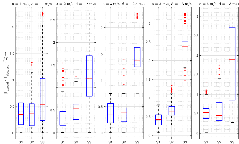
(a) Temperature (T). (S1—P1XQ2 (housing), S2—P1Nimbus2 (housing), and S3—P1Nimbus1 (no housing))
