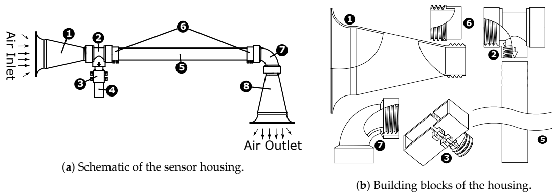
Figure 4. ① Inlet, ② Housing-Sensor Holder Coupler, ③ iMet XQ2 Sensor Adapter, ④ iMet XQ2 sensor, ⑤ Carbon Fiber Tube, ⑥ Carbon Fiber Tube Adapter, ⑦ L-bend, and ⑧ Outlet.
