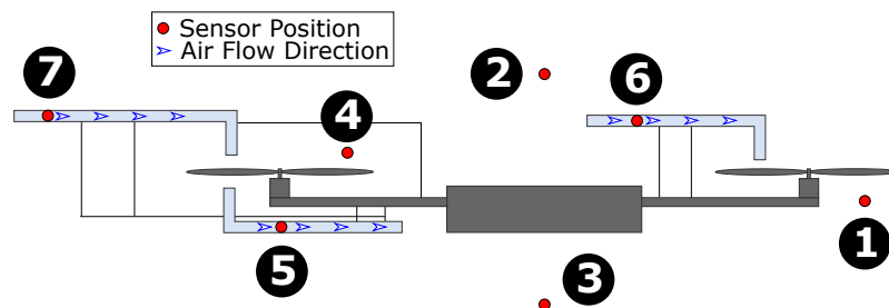
Figure 2. A schematic of the different Sensor Placement Configurations: 1 Direct Downwash, 2 Over the UAS, 3 Under the UAS, 4 Direct Upwash, 5 Downwash housing, 6 Upwash Housing with Inlet Pointed Inside, and 7 Upwash Housing with Inlet Pointed Outside.
