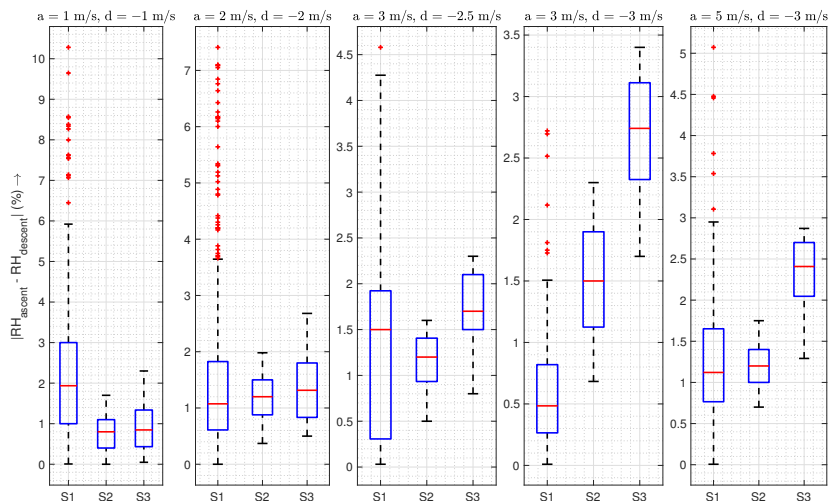
(b) Humidity (RH). (S1—P1XQ2 (housing), S2—P1Nimbus2 (housing), and S3—P1Nimbus1 (no housing))
