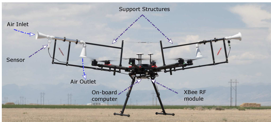
Figure 1. A field trial of sensor housings mounted on a DJI M600 Pro UAS using the square carbon-fiber tube support structure.
