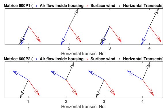
Figure 12. The figure shows the air flow, surface wind, and transect direction during each of the four transect flights conducted during each of the three horizontal flights through the inversion layer.
