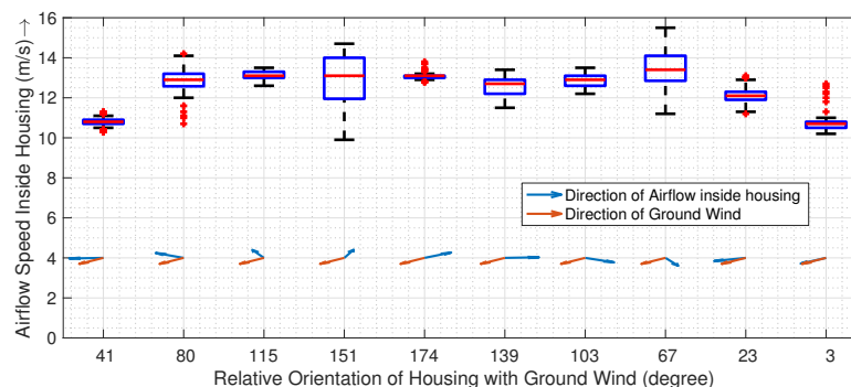
Figure 6. The plot shows a sensitivity in the airflow speed inside the housing in the presence of wind for 10 consecutive flights at different orientations of the UAS from the north at a ground wind speed of 6 mph from the northeast. The box plot captures the 25th to 75th percentile of data, while the central red line indicates the median. The black whiskers and the red plus signs indicate the extreme range and outliers respectively.
