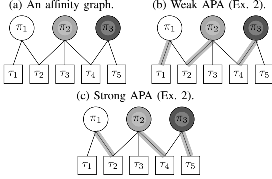
Fig. 1: Affinity graph examples.
