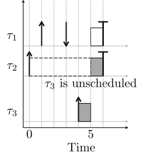
Fig. 5: NP execution (denoted with dashes) breaks progression.
