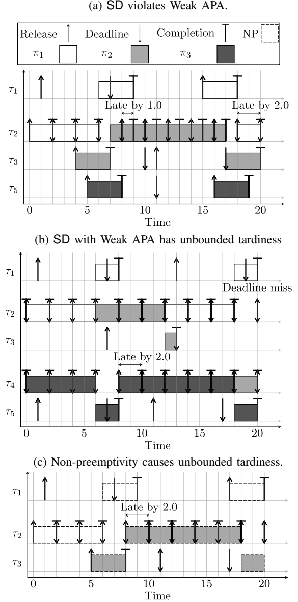
Fig. 2: Bounded tardiness counterexamples. (Longer versions are available online [10].)
