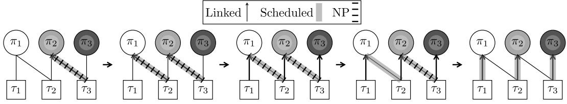
Fig. 7: Example of simultaneous NP blocking.
