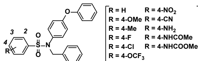
Figure 2. N -Benzylbenzenesulfonamide compounds exhibiting GR antagonistic activity.
