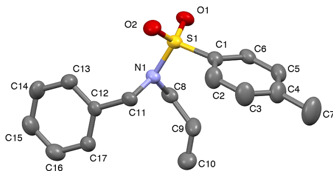
Figure 3. The molecular structure of N -allyl- N -benzyl-4-methylbenzenesulfonamide ( 3b ) with atom labeling scheme. Displacements of ellipsoids are shown at the 50% probability level. Hydrogen atoms have been omitted for clarity.
