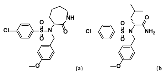
Figure 1. 2-[( N -Benzyl- N -phenylsulfonamido)alkyl] amide derivatives reported to exhibit inhibition against \gamma -secretase. The compounds shown are ( R )-2-[(4-chlorobenzensulfonyl)-(4-methoxybenzyl)amino]-2-hexanolactam (a) and ( R )-2-[(4-chlorobenzensulfonyl)-(4-methoxybenzyl)amino]-4-methylpentanoic acid amide (b).
