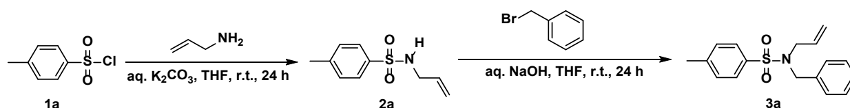
Scheme 1. Synthesis of N -allyl-4-methylbenzenesulfonamide (2a) via the treatment of 4-methylbenzenesulfonyl chloride (1a) with allylamine and the benzylation of compound 2a to form N -allyl- N -benzyl-4-methylbenzenesulfonamide (3a).
