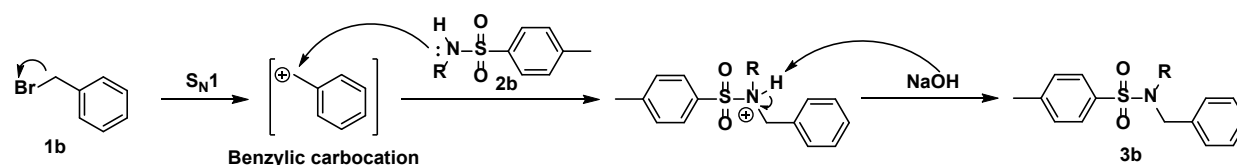
Scheme 2. A proposed S N 1-like mechanism for the benzylation of primary amine derived from 4-methylbenzenesulfonamides.
