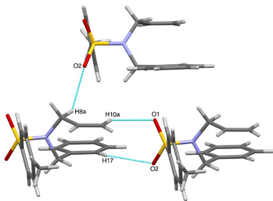
Figure 4. A depiction of the intermolecular hydrogen bonds in the crystal structure of N -allyl- N -benzyl-4-methylbenzenesulfonamide shown as capped sticks with standard CPK colors. Hydrogen bond contacts are depicted with cyan dashed lines. Atom labels follow the atom numbering scheme in Figure 3.
