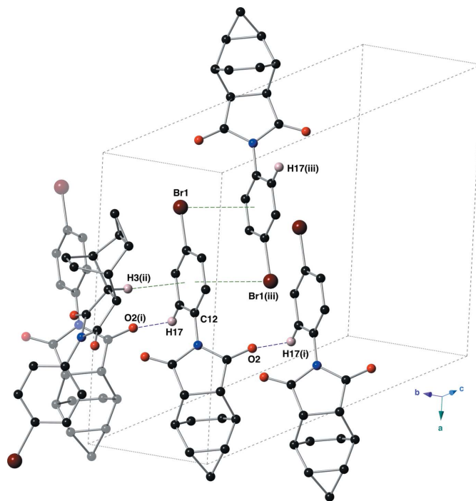
Figure 6 Non-covalent interactions present in the crystal of imide II , using a ball-and-stick model. Only those hydrogen atoms involved in an interaction are shown for clarity. C–H \cdots O hydrogen bonds are shown with purple, dashed lines, while C–H \cdots\pi and C–Br \cdots\pi interactions are shown with green, dashed lines. Symmetry codes: (i) x, y-1, z ; (ii) -x+\frac{1}{2}, y+\frac{1}{2}, -z+\frac{3}{2} .
