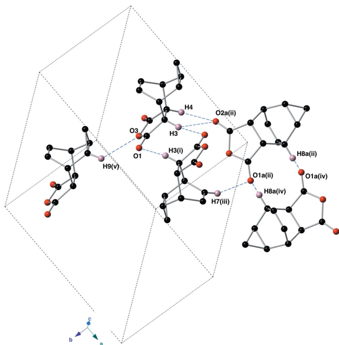
Figure 5 Depiction of the C–H \cdots O hydrogen bonds (blue, dashed lines) present in the crystal of anhydride I , using a ball-and-stick model. For clarity, only those hydrogen atoms involved in an interaction are shown. Symmetry codes: (i) -x+2, -y+1, -z ; (ii) x+1, y, z ; (iii) -x+1, -y+1, -z ; (iv) -x+1, -y+2, -z ; (v) x, y+1, z .
