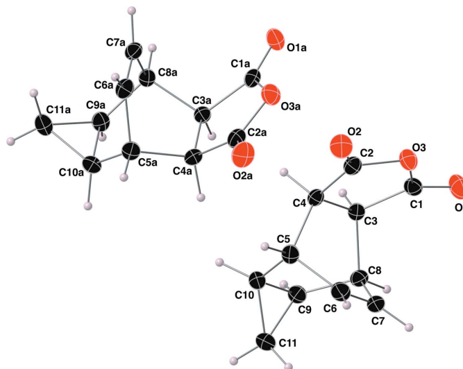
Figure 3 The molecular structure of the anhydride I , with the atom-labeling scheme for both crystallographically unique molecules. Displacement ellipsoids are shown at the 40% probability level using standard CPK colors.
