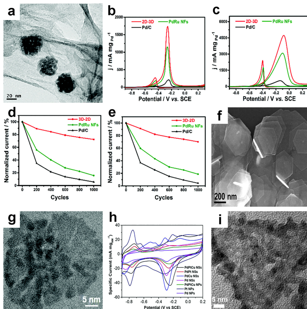
Fig. 4. (a) TEM image of 3D – 2D PdRu/NiZn oxyphosphide nanohybrids. CV curves of 3D – 2D nanohybrids, 3D PdRu NFs, and Pd/C in (b) 1 M KOH + 1 M CH 3 OH, and (c) 1 M KOH + 1 M CH 3 CH 2 OH at the scan rate of 50 mV s -1 . Long-term stability comparison of 3D – 2D nanohybrids, 3D PdRu NFs, and Pd/C for 1000 potential cycles toward (d) MOR and (e) EOR. (f) SEM image of PtSn nanosheets. (g) High-magnification TEM image of the ultrathin PdPtCu nanosheets. (h) CV curves of the trimetallic PdPtCu nanosheets, bimetallic PdPt and PdCu nanosheets, monometallic Pd nanosheets, PdPtCu nanoparticles, and commercial Pt and Pd nanoparticles in 1.0 M KOH at 50 mV s -1 . (i) Typical TEM image of porous PtAg nanosheets. (a-e) Reproduced from Ref. [54] with permission from The Royal Society of Chemistry. (f) Reprinted from Ref. [55], Copyright (2018), with permission from Elsevier. (g, h) Reproduced from Ref. [82] with permission from The Royal Society of Chemistry. (i) Reprinted from Ref. [83], Copyright (2018) Springer Nature.
