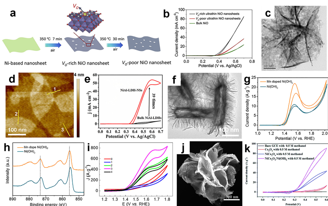
Fig. 5. (a) Schematic illustration for the fabrication of V_{O} -rich/poor ultrathin NiO nanosheets. (b) CV curves of the various NiO samples in 1 M KOH + 0.5 M CH_3OH . (c) TEM image of NiCo_2O_4 . (d) AFM topograph of NiAl-LDH nanosheets. (e) CV curves of bulk NiAl-LDHs and NiAl-LDH nanosheets modified electrodes in 1.0 M NaOH + 1.0 M ethanol at the scan rate of 50\text{ mV s}^{-1} . (f) TEM image of the hollow Mn-doped Ni(OH)_2 nanostructures. (g) CVs of hollow Mn-doped Ni(OH)_2 nanostructures and Ni(OH)_2 nanosheets modified electrode in 1 M KOH + 0.5 M CH_3OH at the scan rate of 50\text{ mV s}^{-1} . (h) XPS spectra of Ni 2p electrons of hollow Mn-doped Ni(OH)_2 nanostructures and Ni(OH)_2 nanosheets. (i) CV curves in nitrogen-saturated 1 M KOH + 3 M CH_3OH . (j) FESEM image of NiCo_2O_4/Ni(OH)_2 . (k) CV curves of GCE (black), Co_3O_4 /GCE (red), NiCo_2O_4 /GCE (blue), and NiCo_2O_4/Ni(OH)_2 /GCE (magenta) in 1 M KOH + 0.5 M CH_3OH at the scan rate of 10\text{ mV s}^{-1} . (a, b) Reprinted from Ref. [92], Copyright (2018), with permission from Elsevier. (c) Reprinted from Ref. [95], Copyright (2014), with permission from Elsevier. (d, e) Reprinted from Ref. [90], Copyright (2017), with permission from Elsevier. (f-h) Reprinted from Ref. [101], Copyright (2018), with permission from Elsevier. (i) Reprinted with permission from Ref. [102]. Copyright (2018) American Chemical Society. (j, k) Reproduced from Ref. [103] with permission from The Royal Society of Chemistry.
