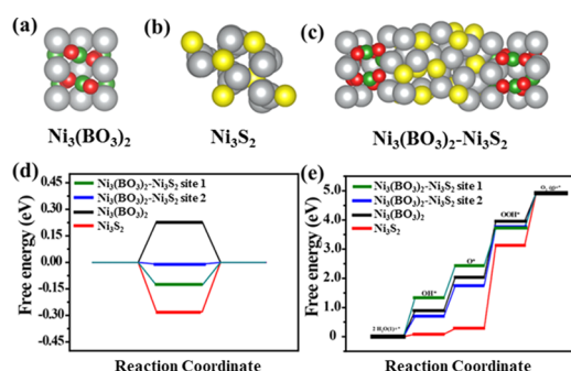
Figure 5. Schematic models of (a) \text{Ni}_3(\text{BO}_3)_2 , (b) \text{Ni}_3\text{S}_2 , and (c) \text{Ni}_3(\text{BO}_3)_2 – \text{Ni}_3\text{S}_2 heterostructures. Gibbs free energy diagram for (d) HER and (e) OER on \text{Ni}_3(\text{BO}_3)_2 , \text{Ni}_3\text{S}_2 , and \text{Ni}_3(\text{BO}_3)_2 – \text{Ni}_3\text{S}_2 heterostructure sites 1 and 2.
