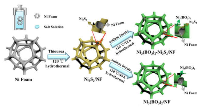
Scheme 1. Schematic Illustration of the Fabrication of the \text{Ni}_3\text{S}_2/\text{NF} , \text{Ni}_3(\text{BO}_3)_2\text{-Ni}_3\text{S}_2/\text{NF} , and \text{Ni}_3(\text{BO}_3)_2/\text{NF} Electrodes
