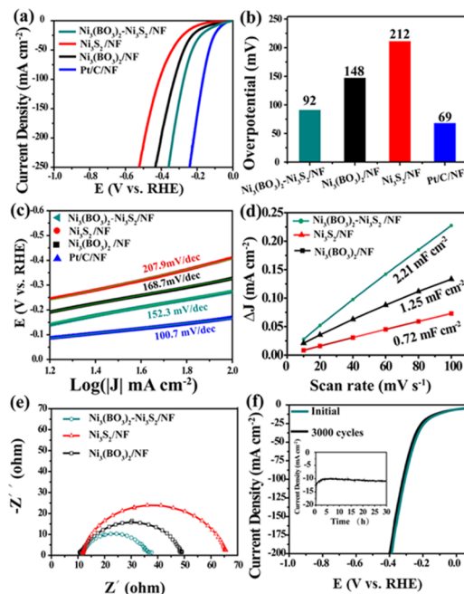
Figure 3. (a) HER polarization curves, (b) HER overpotential ( \eta_{10, \text{HER}} ) at 10 \text{ mA cm}^{-2} , and (c) Tafel plots of \text{Ni}_3\text{S}_2/\text{NF} , \text{Ni}_3(\text{BO}_3)_2\text{-Ni}_3\text{S}_2/\text{NF} , \text{Ni}_3(\text{BO}_3)_2/\text{NF} , and Pt/C/NF. (d) Estimation of C_{\text{dl}} . (e) Nyquist plots of \text{Ni}_3\text{S}_2/\text{NF} , \text{Ni}_3(\text{BO}_3)_2\text{-Ni}_3\text{S}_2/\text{NF} , and \text{Ni}_3(\text{BO}_3)_2/\text{NF} . (f) Polarization curves of \text{Ni}_3(\text{BO}_3)_2\text{-Ni}_3\text{S}_2/\text{NF} in the first scan and after 3000 cycles in 1.0 M KOH. Inset to panel (f) shows the current–time profile at \eta = -85 \text{ mV} in 1.0 M KOH for 30 h.
