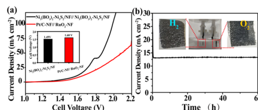
Figure 6. (a) Polarization curves and (b) long-term durability tests at 1.55 V for overall water splitting by \text{Ni}_3(\text{BO}_3)_2 – \text{Ni}_3\text{S}_2 /NF in a 1.0 M KOH solution. Inset to panel (a) is the cell voltage at 10 \text{ mA cm}^{-2} , and inset to panel (b) are the photographs of the electrodes during overall water splitting.
