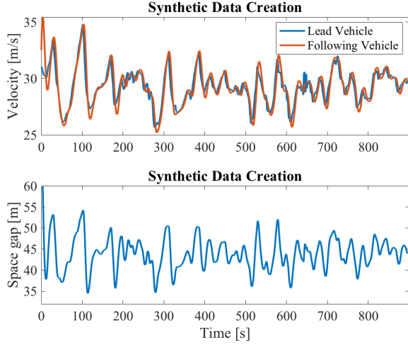
Fig. 1: Synthetic space gap and following vehicle data, generated from an empirical lead vehicle profile.
