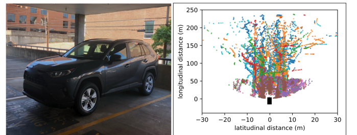
Fig. 4: Left: The 2019 ACC equipped stock SUV used in the experiment. Right: relative position data collected from the CAN bus of the vehicle within a duration of 15 min drive. Each point corresponds to the latitudinal and longitudinal distance to an object detected by the stock radar sensor and reported on the CAN bus. Colors correspond to distinct objects.
