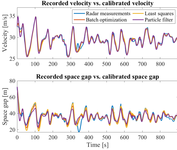
Fig. 7: Comparison between recorded vehicle velocity and space gap vs simulated for each model found.
