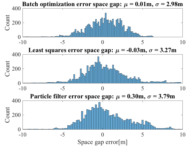
Fig. 9: space gap error distribution for each calibrated model.
