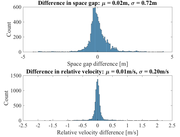
Fig. 6: Histogram of the difference between GPS measurements and CAN bus measurements for space gap and relative velocity measurements.
