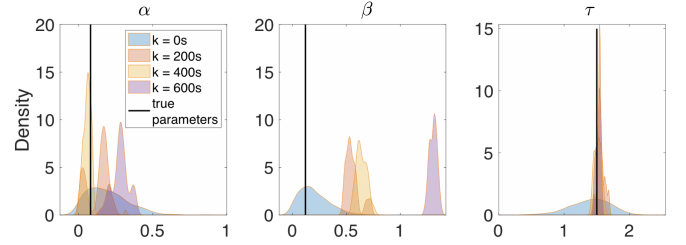
Fig. 2: Posterior parameter PDFs for equilibrium driving dataset from PF estimates. The plot shows that parameter \alpha and \beta are not identified correctly, i.e., the distributions drift away from the true values (black vertical lines) over time. Only the distribution of \tau converges to the true value.
