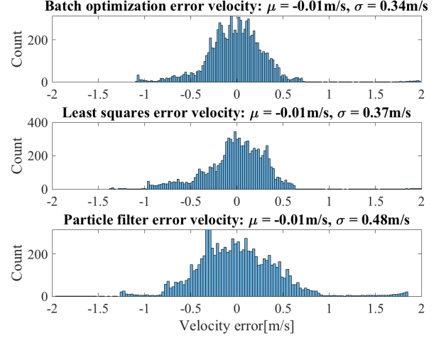
Fig. 8: velocity error distribution for each calibrated model.
