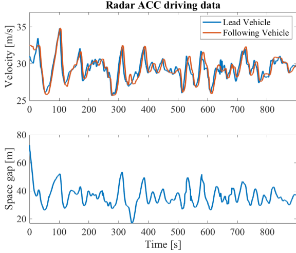
Fig. 5: CAN bus measurement of an ACC-enabled vehicle following a human-driven vehicle.
