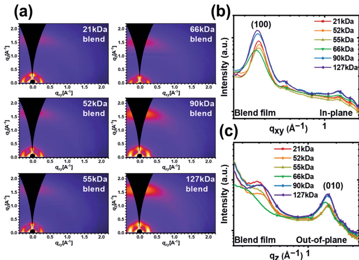
Fig. 8 PNDIBS molecular weight dependence of 2D-GIWAXS data for PBDB-T:PNDIBS blend active layers processed at the optimal conditions: (a) 2D-GIWAXS patterns; (b and c) 1D line cuts of GIWAXS patterns in the in-plane (IP) (b) and the out-of-plane (OOP) direction (c).
