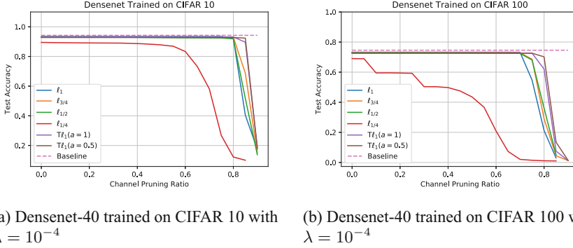
Fig. 4. Effect of channel pruning ratio on the mean test accuracy of five runs of Densenet on CIFAR 10/100. Baseline refers to the mean test accuracy of the unregularized model that is not pruned.
