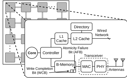
Figure 1. WiSync manycore.
