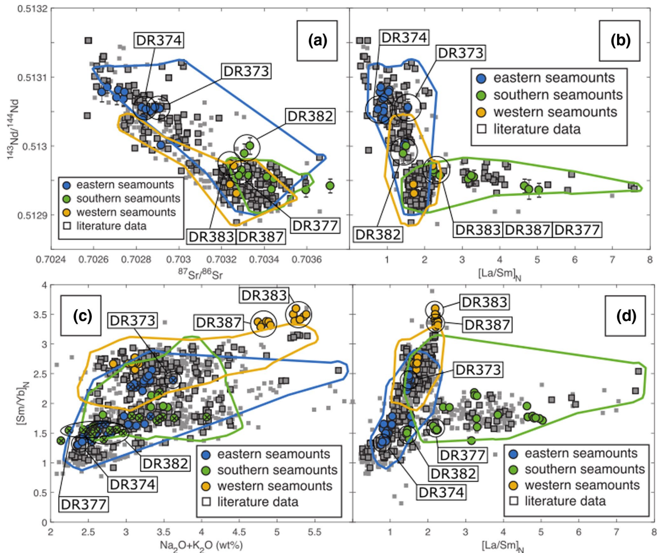
Figure 6. Trace element and Isotopic variation of seamounts compared to previously published data. Seamount samples are shown as colored circles. Colored lines outline data used in the clustering analysis within each region, as defined by the extents of Figure 3 and shown in Figure 1. Gray outlined squares are literature data used in the clustering (see Section 3.5 for references). Smaller gray squares show all other compiled literature data (see Table 1 for references).
