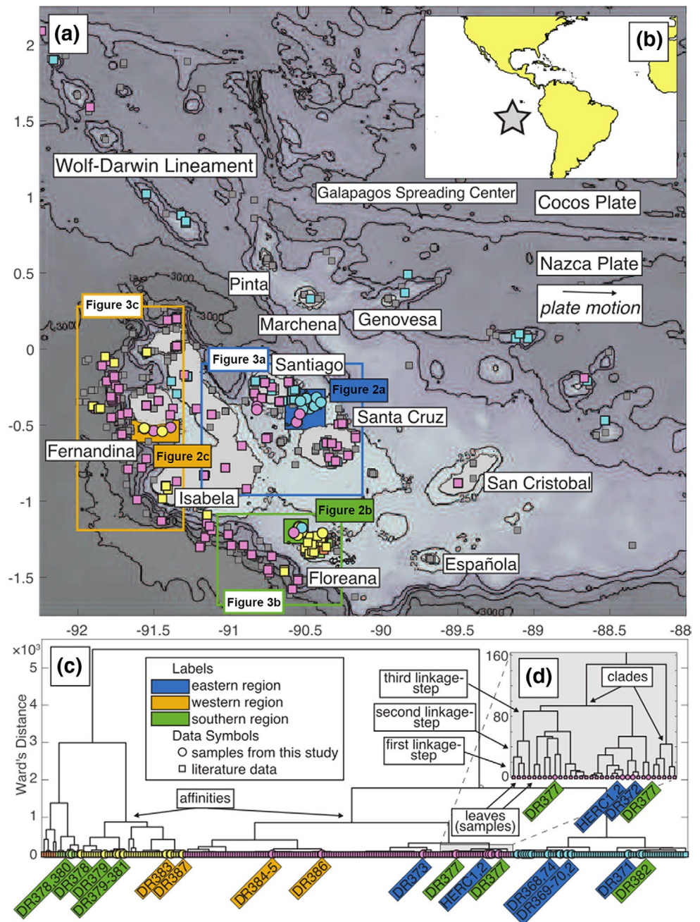
Figure 1. a) Map of the Galápagos Archipelago, with islands are shown in green. Literature sample locations are shown as colored squares (see Section 3.5 for data sources). Samples from this study are shown as colored circles. Samples are colored by agglomerative clustering into five affinities based on similarities in trace element and isotopic ratios (see panel c and Section 3.5 for more details). Samples from literature data that do not include all of the elements and isotope ratios used in the clustering analysis are gray (see Table 1 for data sources). Bathymetric contour interval is 500 m except the shallowest index at 250 m, data from Ryan et al. (2009). Filled colored boxes show the locations of panels in Figure 2. Open colored boxes show the locations of panels in Figure 3. Nazca Plate motion, relative to the fixed hotspot reference frame is nearly due east and is shown as a black arrow in the bottom left of the map (Argus et al., 2010). (b) Gray star shows the location of the Galápagos Archipelago. (c) Dendrogram showing results of the regional agglomerative clustering analysis. Samples from this study are indicated by the color flags corresponding to their regional colors in panel a and labeled by seamount. Samples are ordered by their similarity within each affinity (see Section 3.5 for more details) (d) Select portion of the dendrogram, enlarged to show details. Individual samples are shown as leaves at the bottom of the diagram. The first three linkage-steps for the leaf on the far left of the diagram, and its subsequent clades, are indicated with arrows. Clades are any group of samples within the dendrogram, with examples labeled in the figure inset.
