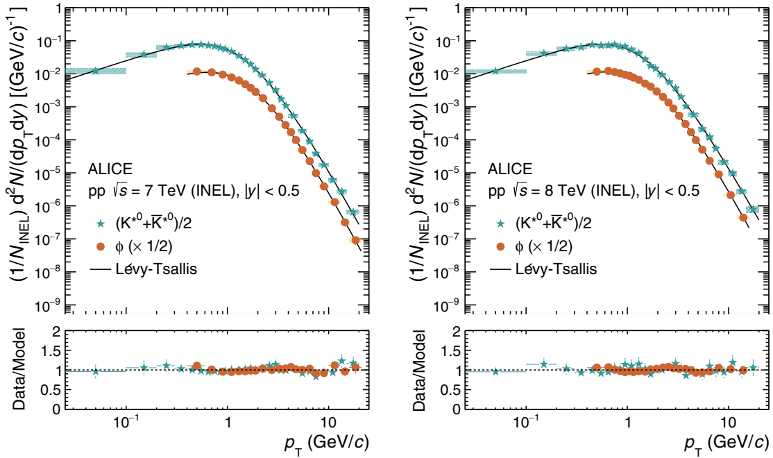
FIG. 2. Upper panels shows the p_T spectra of K^{*0} and \phi in inelastic pp collisions at 7 TeV (left) and 8 TeV (right) and fit with the Lévy-Tsallis distribution [23,24]. The normalization uncertainty in the spectra is ^{+7.3}_{-3.5}\% for 7 TeV and 2.69% for 8 TeV. The vertical bars show statistical uncertainties and the boxes show systematic uncertainties. The lower panels show the ratio of data to the Lévy-Tsallis fit. Here, the bars show the systematic uncertainty.
