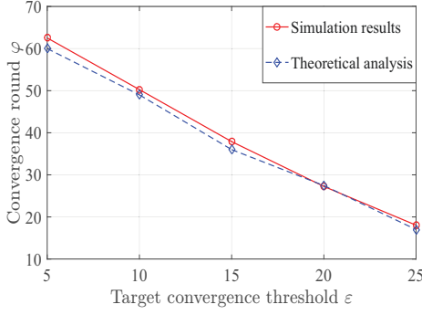
Fig. 2. Validation of Theorem 1.
