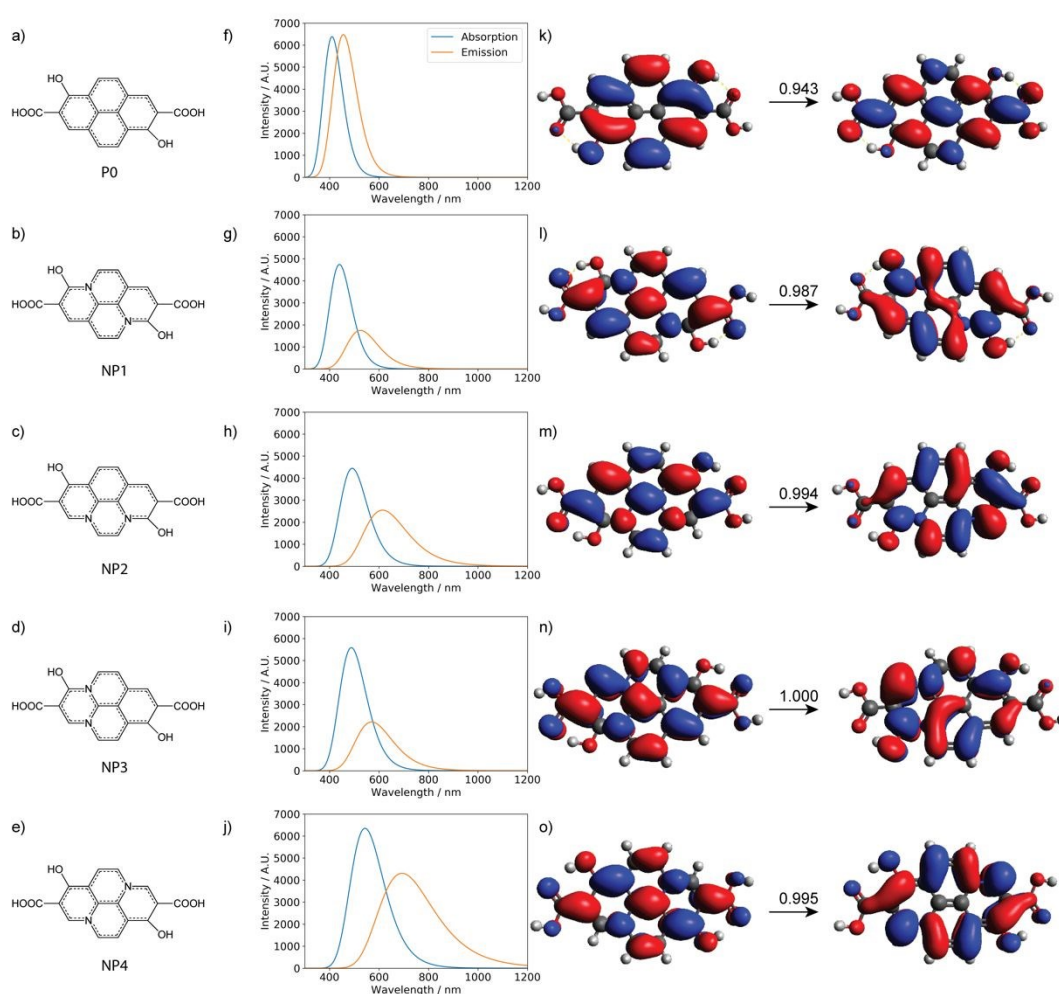
Figure 9. Chemical structures, calculated UV-Vis absorption, fluorescence spectra, and natural transition orbitals (NTOs) for the pyrene-based model. (a-e) The chemical structures of the nitrogen-free system (P0) and nitrogen-doped models (NP1, NP2, NP3, NP4). (f-j) The corresponding absorption and fluorescence spectra calculated at the level of TD- \omega B97XD/6-31+g(d,p). (k-o) The corresponding dominant NTOs.
