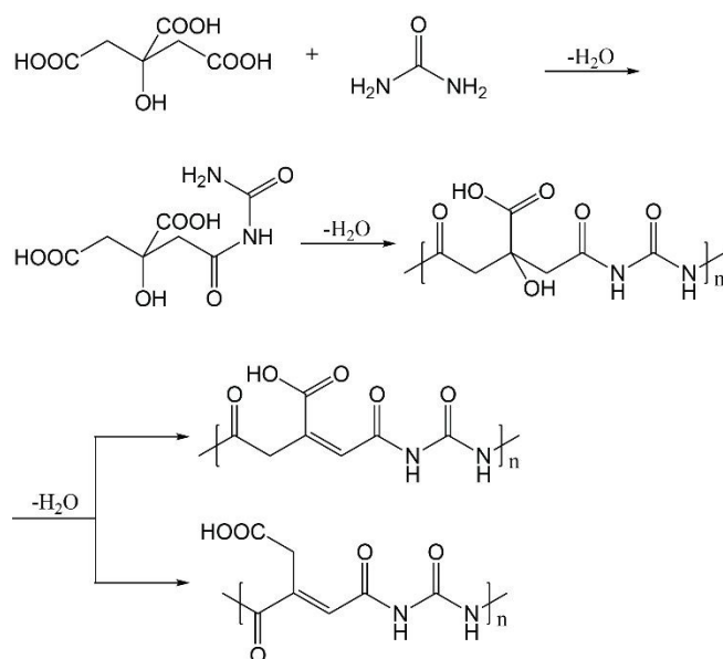
Figure 10. Proposed formation pathway for polyamide and dehydrated polyamide.
