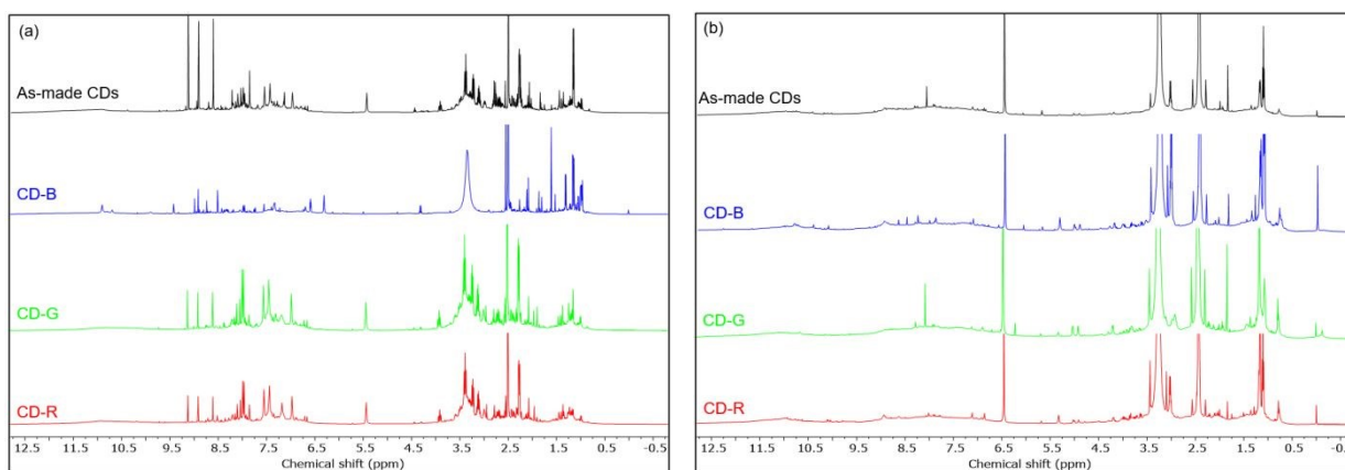
Figure 4. ^1\text{H} NMR spectra of as made CDs, CD-B, CD-G, and CD-R in \text{DMSO-d}_6 before dialysis (a) and after dialysis (b).
