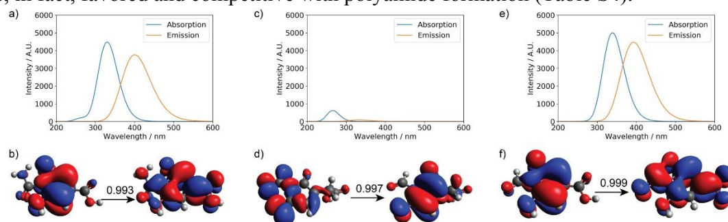
Figure 6. Calculated UV-Vis absorption, fluorescence spectra, and natural transition orbitals (NTOs) of candidate small molecule chromophores (for their structures, see Figure S11). The absorption and fluorescence spectra were calculated at the level of TD- \omega B97XD/6-31+g(d,p) for a) product 1 , c) product 2 , and e) product 3 ; b), d), and f) are the corresponding dominant NTO pairs. Negative values correspond to holes in red, and positive values correspond to particles in blue. To generate the absorption/emission line shapes in this and subsequent figures, a line width of 0.4 eV (default in Gaussview) was used; for absorption, we consider the three lowest excited states, while for emission, we consider only the first excited state.
