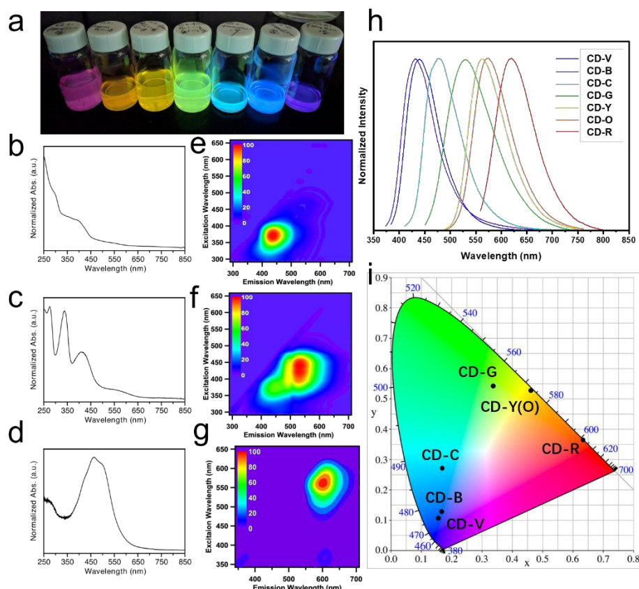
Figure 1. (a) Photograph of obtained CD fractions illuminated by UV light, (b)-(d) UV-vis extinction spectra and (e)-(g) 2D EEM of CD-B, CD-G, and CD-R, (h) the normalized fluorescence spectra and (i) the chromaticity diagram of CD fractions (CD-Y and CD-O overlaps).
