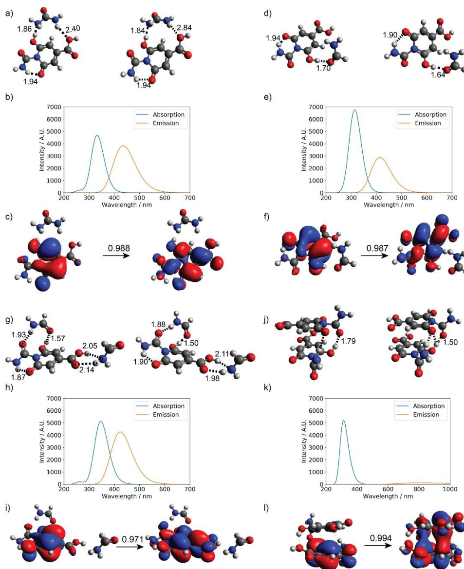
Figure 7. Hydrogen-bonding effect on the photoactivity of small molecule chromophore 1 (see Figure S11 for structure). Optimized geometries at the ground state and first excited state: a) urea and product 1 , d) formamide and product 1 , g) two formamide and product 1 , and j) stacked dimer of product 1 ; b), e), h), and k) are corresponding absorption and fluorescence spectra computed at the level of TD- \omega B97XD/6-31+g(d,p); c), f), i) and l) are corresponding dominant NTO pairs. Negative values correspond to holes in red, and positive values correspond to particles in blue.
