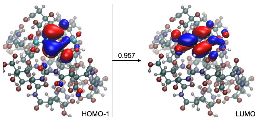
Figure 8. An example for the structure of a small molecule chromophore surrounded by a decamer polyamide. Also shown is the nature of the excitation, which largely involves excitation from HOMO-1 to LUMO with an amplitude of 0.957. Calculations at LC-TD-DFTB2 and TD- \omega B97XD levels are consistent in the nature of excitation (see Table S10 for details).
