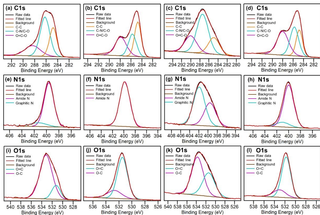
Figure 3. High resolution C 1s, N 1s and O 1s XPS spectra for raw as-synthesized CDs (a, e, i), blue CDs (b, f, j), green CDs (c, g, k) and red CDs (d, h, l).
