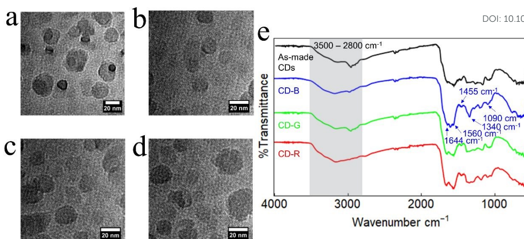
Figure 2. TEM images of (a) as-made CDs, (b) CD-B, (c) CD-G, and (d) CD-R. (e) FT-IR spectra of as-made CDs and CD-B, CD-G, and CD-R.
