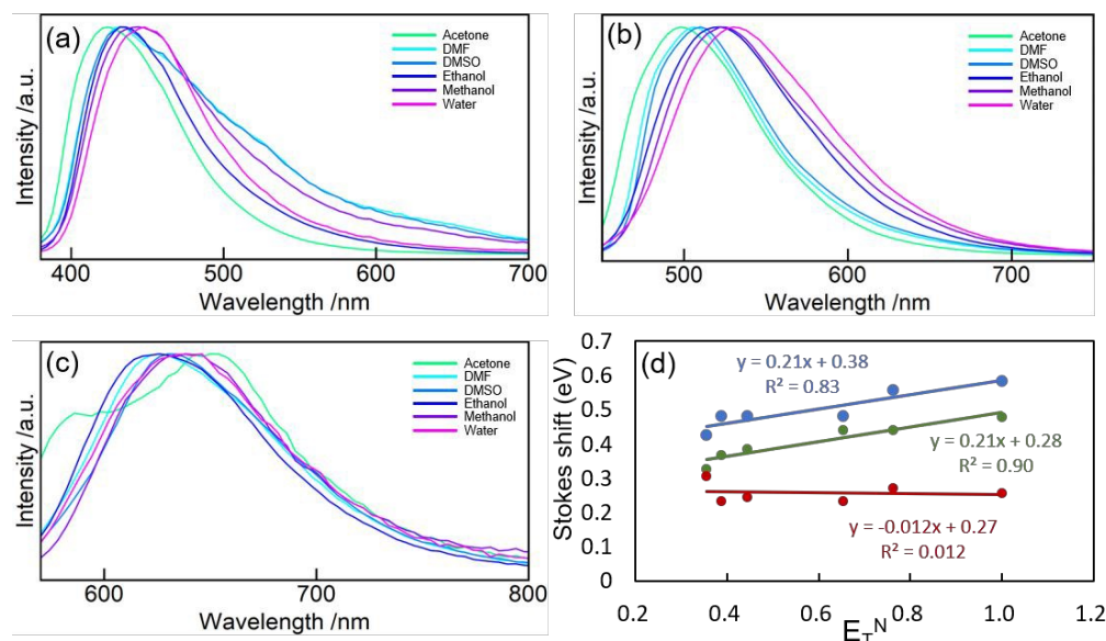
Figure 5. PL spectra of CD-B (A), CD-G (B), and CD-R (C) dispersed in acetone, DMF, DMSO, ethanol, methanol, and water. (D) Stokes shift of CD-B, CD-G, and CD-R plotted against E_T^N .
