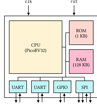
Figure 2. A schematic of NOTARY’s agent domain SoC, which is formally verified to satisfy deterministic start.
