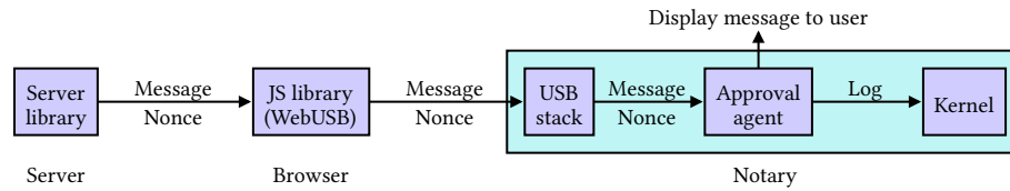
Figure 4. Approval agent framework: server asks the user to approve an operation by sending a message describing the operation through the browser to the approval agent on NOTARY, which displays it to the user. If the user approves, the approval agent signs the message and logs it. The signed response (not shown) is returned to the server through the same path.
