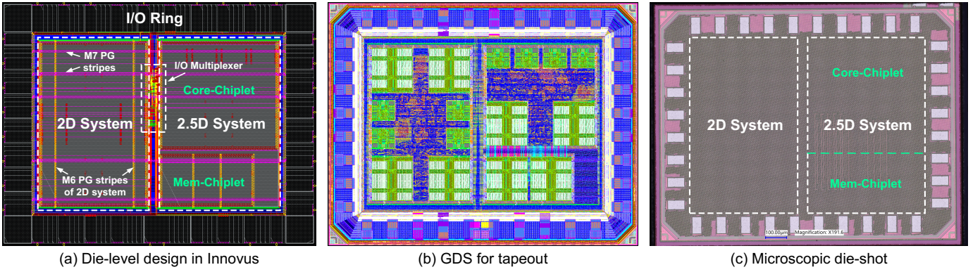
Fig. 9. Final design for tape-out and the fabricated die: (a) Die-level design, (b) Combined GDS for tape-out, (c) Microscopic image of the taped-out die.
