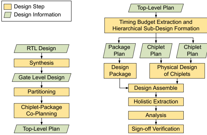
Fig. 4. Overall CAD flow for 2.5D system design
