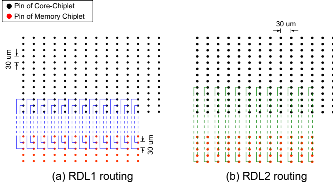
Fig. 5. 2.5D package routing generated by the RDL planner tool
