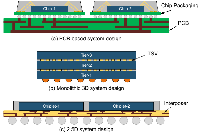
Fig. 1. System Design technologies: (a) PCB based system (b) TSV based monolithic 3D system (c) High density 2.5D integration scheme
