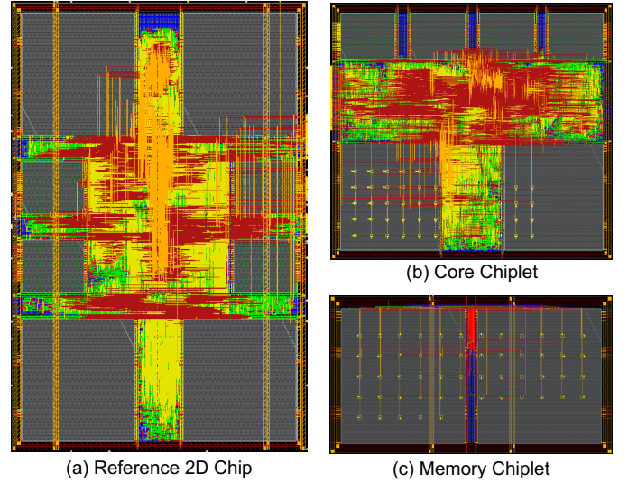
Fig. 6. Layouts of the reference 2D chip and the chiplets for 2.5D integration
