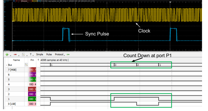
Fig. 8. Chip testing waveforms from logic analyzer
