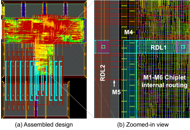
Fig. 7. Finished 2.5D Design: (a) Innovus view after Design Assemble (b) Zoomed-in view showing package and chiplet routing
