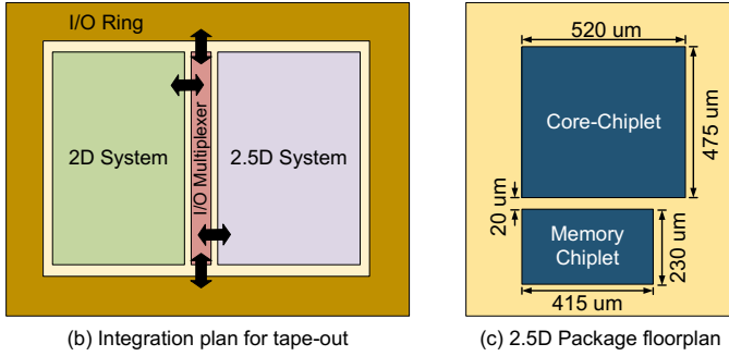
Fig. 2. (a) Architecture of the ARM Cortex-M0 micro-controller system (b) Integration floorplan for shared-block system design (c) Package floorplan generated by RDL planner tool
