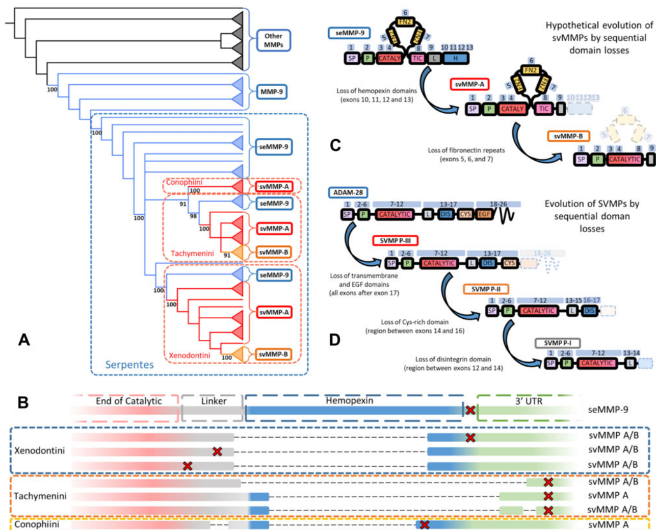
Fig. 4. Evolution of svMMPs. (A) Schematic ML tree of vertebrate MMPs, seMMP-9s, and svMMPs showing the phylogenetic relationships between the three types of proteins (the complete phylogenetic trees are supplied in supplementary figs. S2 and S3, Supplementary Material online). Dashed boxes indicate relevant taxa. Independent origins could be assumed at least for Xenodontini and Tachymenini, as svMMPs from these groups cluster with their endogenous seMMP-9. Bootstrap support values shown for relevant nodes were estimated from the full-length CDS analysis. (B) Schematic representation of the C-terminal part and 3'-UTRs of svMMPs from the three tribes aligned against their endogenous counterparts (the complete alignments are supplied in supplementary figs. S4–S6, Supplementary Material online). Red marks indicate the position of the stop codon in each protein. The svMMP type (A or B) in which each pattern was found is specified to the right. (C) Proposed evolution of svMMPs through sequential domain losses. Numbered boxes over the protein domains of seMMP-9 represent the exons coding them, based on the reported MMP-9 gene from Python bivittatus (Gene ID: 103064710). For svMMP-A and svMMP-B, the numbered boxes represent the exons expected to code for the domains, numbered according to the seMMP-9 gene. (D) Sequential domain losses via exon shuffling previously suggested to have occurred during SVMP evolution from ADAM28 ( Sanz et al. 2012; Giorgianni et al. 2020 ), indicating a similar trend toward a simplified derived structure.
