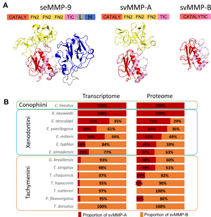
Fig. 2. The three types of MMPs found in snake venoms: one endogenous MMP-9 (seMMP-9) and two venom-specific MMPs (svMMP-A and svMMP-B). (A) Structural comparison between the three different types of MMPs identified in snake venom glands. Domains described in the linear model are: CATALY (first portion of catalytic), FN2 (fibronectin), TIC (second part of catalytic), L (linker), and H (hemopexin). 3D structures of seMMP-9, svMMP-A, and svMMP-B were modeled by homology using the SWISS-MODEL online platform on default parameters. The templates used were 1L6J (Elkins et al. 2002) for svMMP-A and B, and theoretical model 1LKG (https://www.modelarchive.org/doi/10.5452/ma-coftn, last accessed August 3, 2020) for seMMP-9. (B) Proportion of both types of svMMP, in both the venom gland transcriptome and the venom proteome, for one species of Conophiini, six species of Xenodontini, and seven species of Tachymenini.
