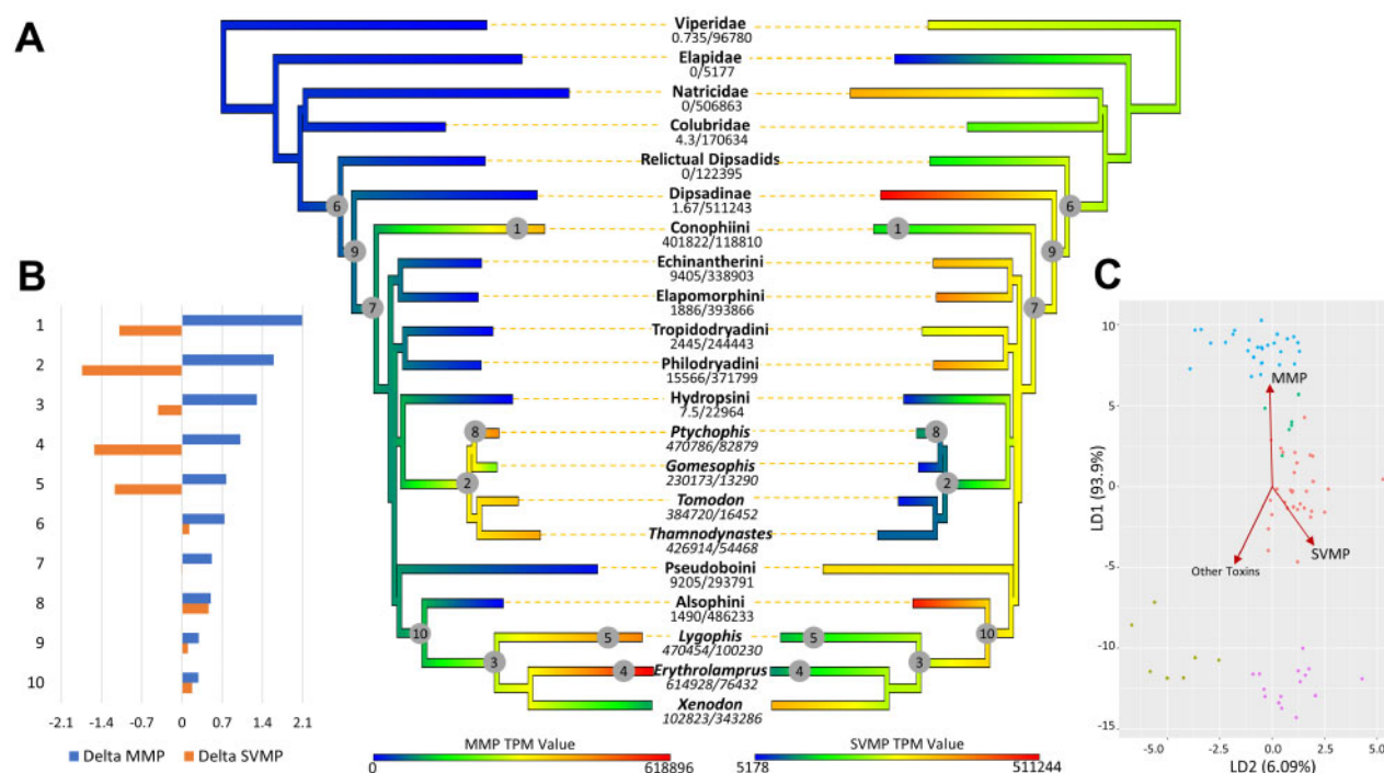
FIG. 5. The balance of venom metalloproteinases during evolution. (A) Ancestral state reconstruction of both MMP (left) and SVMP (right) across several snake groups. Blue branches indicate low expression levels, whereas branches tending to red indicate high expression levels. Mean expression values in TPM for MMPs/SVMPs are shown under each group name. Numbered lineages represent nodes or terminals with the highest MMP expression fold-change in comparison to the previous node. (B) The rank of top ten lineages according to the log2 fold-change of MMP expression levels (blue bars) in comparison to that of the preceding node; SVMP fold-change is also shown (orange bars). (C) LDA analysis showing how changes in MMP and SVMP expression levels are the major drivers in the differentiation of venom gland expression patterns. svMMP and SVMP-positive taxa group in five different clusters: 1) svMMP-rich venoms (blue): constituted by species from Tachymenini, most Xenodontini and Conophiini; 2) svMMP-rich venoms with high level of SVMP expression (green): species of Xenodon (Xenodontini); 3) SVMP-rich venoms with some marked expression levels of svMMP or seMMP-9 (red): species from other tribes of Xenodontinae; 4) SVMP-rich venoms (purple): species from other Dipsadidae subfamilies, Natricidae, some Colubridae and species of Bothrops ; and 5) Venoms rich in other toxins (pistachio): species from Elapidae, Hydropsini, Mastigodryas , and Crotalus .
