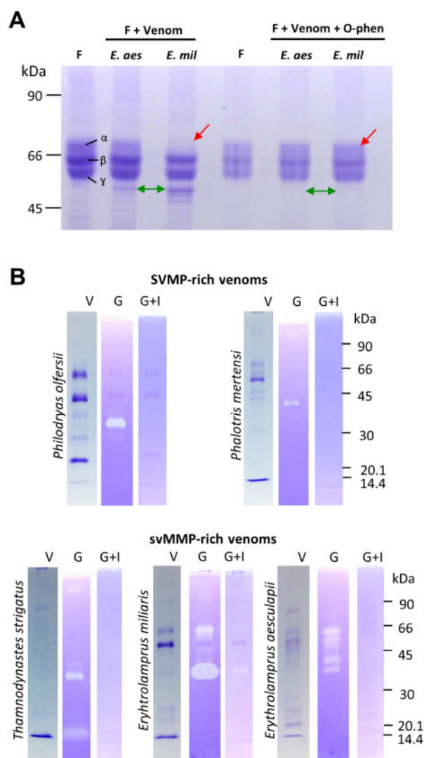
FIG. 6. Metalloproteolytic activities of Xenodontinae venoms. (A) Fibrinolytic activity of E. aesculapii ( E. aes ) and E. miliaris ( E. mil ) venoms over fibrinogen (F) in the absence or presence of the metalloproteinase inhibitor O-phenanthroline (O-phen). Fibrinogen alpha, beta, and gamma chains are indicated in the first lane. Single-headed arrows indicate bands of alpha chain that were visibly degraded when the inhibitor was not added. Double-headed arrows indicate degradation products, which are absent when the inhibitor was added. (B) Gelatinolytic activity assay of SVMP-rich venoms (upper panel) or svMMP-rich venoms (lower panel). V, Venoms from the species indicated on the side run in SDS-PAGE (without gelatin); G, Gelatinolytic activities of the same venoms run in SDS-PAGE polymerized with gelatin; G + I, Gelatinolytic activities of the same venoms run in SDS-PAGE polymerized with gelatin, and in the presence metalloproteinase inhibitor EDTA.
