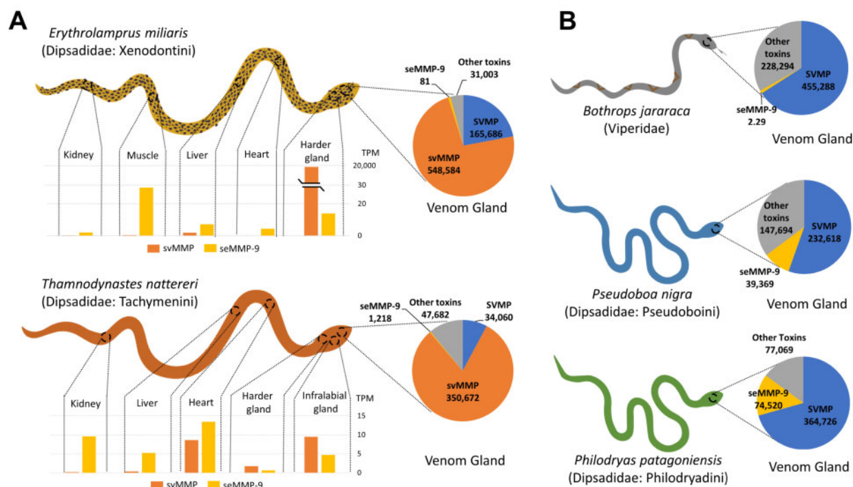
FIG. 3. Expression of putative toxins and MMPs in snake transcriptomes. (A) Expression levels of seMMP-9s and svMMPs in the transcriptomes of various tissues of representative species of svMMP-positive snakes. Note that svMMPs (orange bars and slices) may be detected in restricted amounts in other tissues but are only highly expressed in venom glands. (B) Comparison of the putative toxin proportions in the venom gland transcriptomes of representative species of svMMP-negative snakes. Note an increased proportion of seMMP-9 (yellow slice) in Dipsadidae. All expression values are expressed in TPM.
