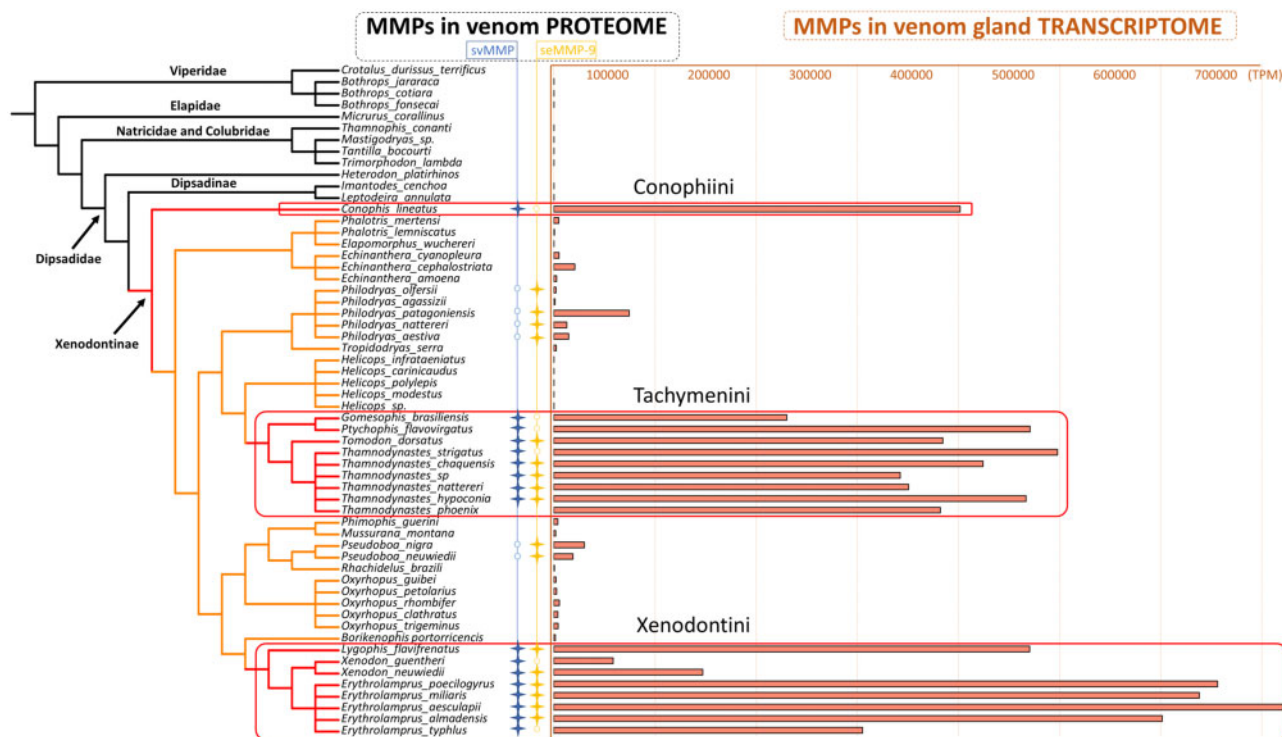
FIG. 1. Occurrence of MMP-9-like transcripts and proteins across snake phylogeny. In the right panel, the red bars represent the average transcripts per million (TPM) value for total MMPs (svMMPs and/or seMMP-9) for each sampled species. The three tribes with MMPs in high abundance are highlighted within a red box; in these cases, the expression values correspond to the total amount of svMMPs and seMMP-9s detected together in the initial screening. For the species outside the boxes, no svMMP sequence was identified and the expression values correspond to seMMP-9 solely. In the columns, blue and yellow crosses indicate the presence in the venom of svMMP and seMMP-9, respectively, detected by proteomics. An open circle indicates that the venom was tested but the protein was not identified (for all other species without marks, the venom was not tested).
