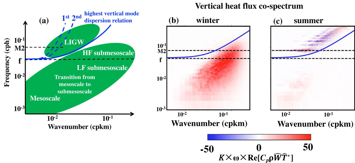
Figure 6. (a) Schematic representation of oceanic motions in frequency-wavenumber space (given as cycles per hour, cph, and cycles per km, cpkm). LIGW denotes linear internal gravity waves; M2 denotes the M2 tidal frequency; f is the Coriolis frequency. The IGW dispersion relations are indicated by blue curves; the first, second, and highest vertical modes are plotted. (b) Frequency-wavenumber cospectrum of the vertical heat flux at 40-m depth during winter (January–March) and (c) summer (July–September), within the Kuroshio Extension region (black dashed box in Figure 3a). The cospectra density ( \text{Re}[C_p \rho \widehat{W} \widehat{T}^*] , unit: \text{W m}^{-2} \text{cph}^{-1} \text{cpkm}^{-1} ) are shown in a variance preserving form; that is, they are multiplied by the wavenumber and frequency to compensate for logarithmic shrinking on both axes. The blue curves show the IGW dispersion curve for the tenth baroclinic mode—the highest resolved by the simulation (Torres et al., 2018).
