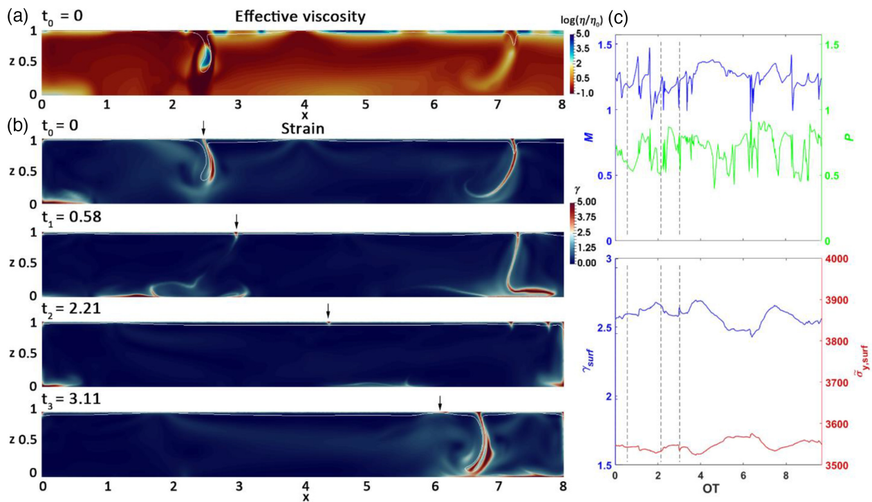
Figure 7. Spreading centre initiation for a model with a high critical strain \gamma_{cr} (18) and low healing timescale B (0.3622). (a and b) Initial effective viscosity \eta and time evolution of the strain \gamma . (c) Top: Time-series of the mobility ( M – dark grey, blue) and plateness ( P – light grey, green). Bottom: Time-series of the surface-averaged strain ( \gamma_{surf} – top line) and surface yield stress ( \sigma_{y,surf} – bottom line; see online version for colour).
