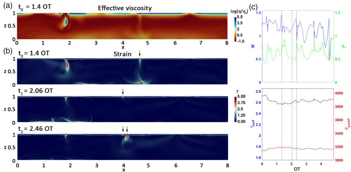
Figure 6. ‘Failed’ subduction initiation for the same model as shown in Fig. 3 with a low healing timescale B (0.3622) and high critical strain \gamma_{cr} (10). (a and b) Initial effective viscosity \eta and time evolution of the strain \gamma . (c) Time-series of (at the top) mobility ( M – dark grey, blue), plateness ( P – light grey, green) and (at the bottom) surface-averaged strain ( \gamma_{surf} – top line) and surface yield stress ( \sigma_{y,surf} – bottom line; see online version for colour).
