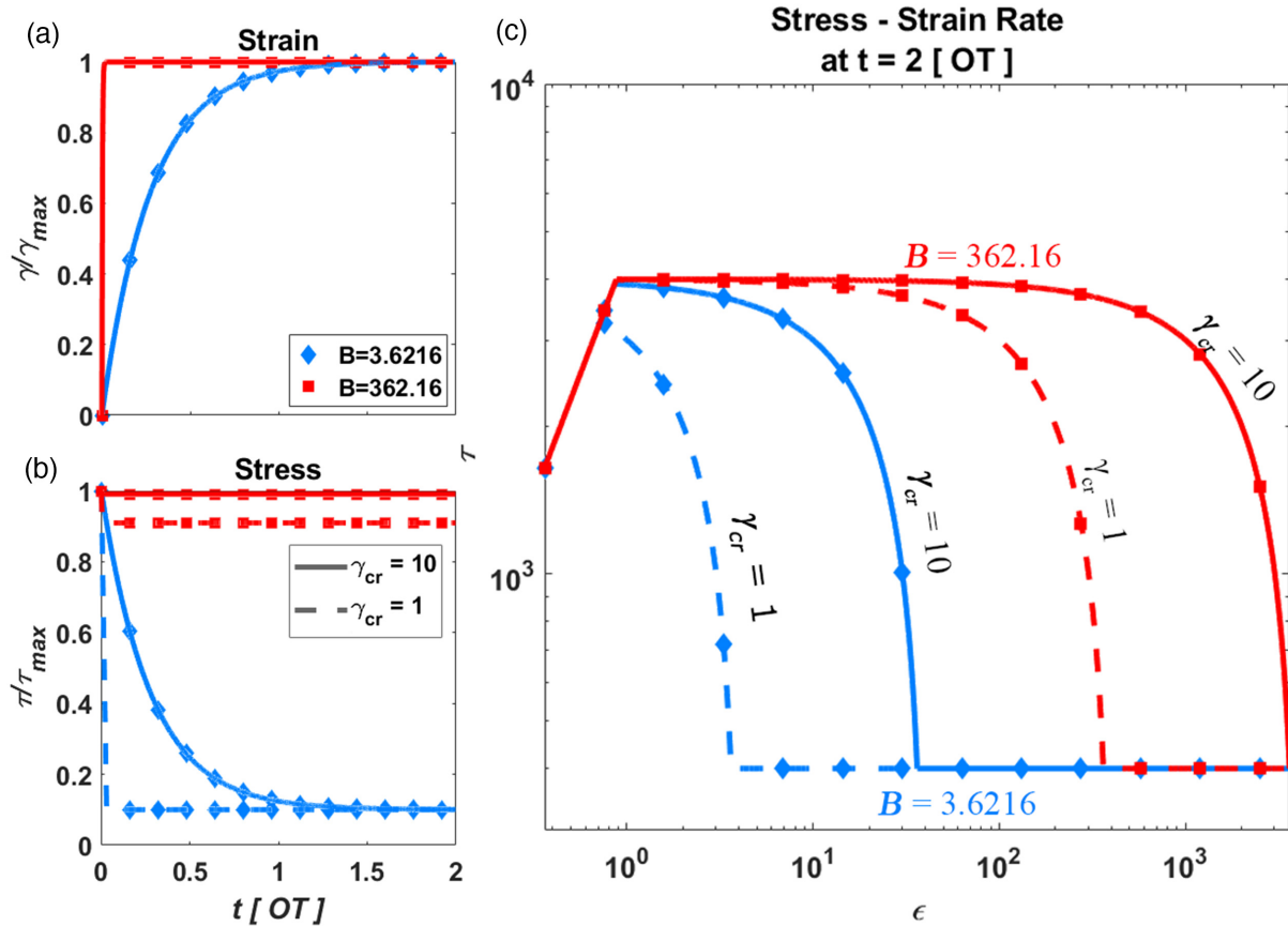
Figure 2. Deformation map for damage weakening rheology assuming a constant strain rate over a duration of 2 OT. (a) Evolution of strain (scaled by \gamma_{\max} ) for different healing timescales B . (b) Evolution of stress (scaled by \tau_{\max} ) for different healing timescales B (squares/red and diamond/blue) and critical strains \gamma_{cr} (solid and dashed). The “undeformed” yield stress is 4 \times 10^3 . (c) Stress–strain rate relation for a range of B and \gamma_{cr} for constant strain rates \dot{\epsilon} after a total time of t = 2 OT. A higher B and \gamma_{cr} result in less accumulated strain and weakening, thus the yield stress is reduced only slightly. A stronger weakening due to lower B and \gamma_{cr} results in stronger reduction in yield stress (see online version for colour).
