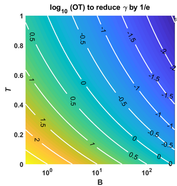
Figure 1. Strain reduction time (background colour and solid contour lines) to reduce \gamma by a factor of 1/e for different temperature and healing timescales. The time is calculated using eq. (8) assuming no deformation is active, that is, the strain-rate is zero. If T = 1 , the total healing rate H is equal to the healing timescale B and thus the reduction time is 1/B . With decreasing T , the healing rate decreases as well and the reduction time increases to c/B , where c is a temperature-dependent constant (see eq. 9 for more detail; see online version for colour).
