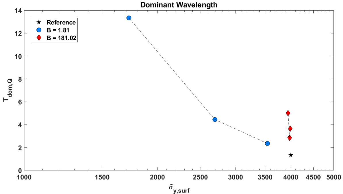
Figure 10. Dominant wavelength of total surface heat flow for models including strain-dependent weakening (SDW) for Ra_Q = 10^6 and \sigma_{y,0} = 4 \times 10^3 (Reference model without SDW) and different healing timescales B and critical strains \gamma_{cr} = 10, 3.6, 2 . In general, SDW shift convection to longer periods and with more dominant weakening (i.e. decreasing \gamma_{cr} ) increases the dominant convection wavelength further (see online version for colour).
