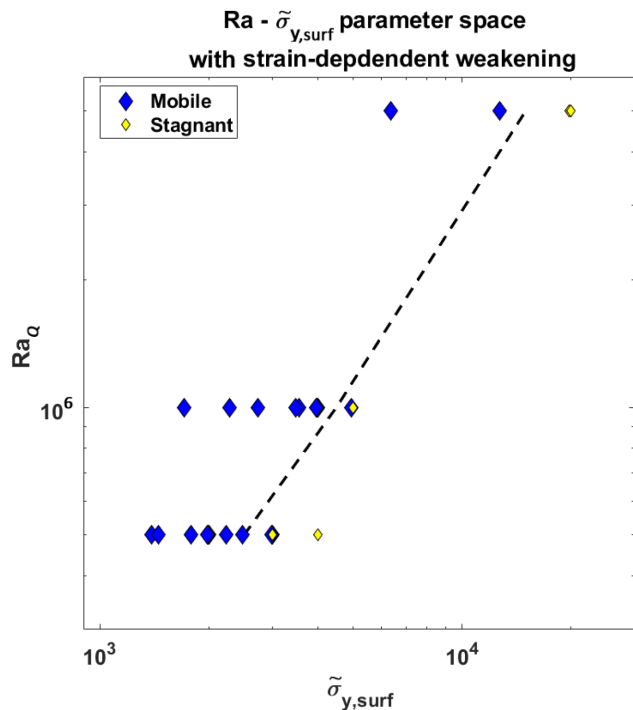
Figure 11. Ra_Q - \sigma_{y,0} parameter space for models with strain-dependent weakening (SDW). The black dashed line indicates the transition between mobile (large diamonds) and stagnant-lid (small diamonds) convection for models without SDW. For models including SDW, we chose a model in a mobile stage adjacent to the boundary as initial condition and increased the yield stress step wise, that is, Ra_Q = 5 \times 10^5 , \sigma_{y,0} = 2 \times 10^3 , 3 \times 10^3 , 4 \times 10^3 ; Ra_Q = 10^6 , \sigma_{y,0} = 4 \times 10^3 , 5 \times 10^3 ; Ra_Q = 5 \times 10^6 , \sigma_{y,0} = 2 \times 10^4 . For each of those Ra_Q - \sigma_{y,0} combinations, we run six models using a certain parameter combination for B and \gamma_{cr} ( B = 1.81, 181.02 ; \gamma_{cr} = 10, 3.6, 2 ). A model is considered stagnant if the mean of the mobility over the full model time is less than 0.1 (see online version for colour).
