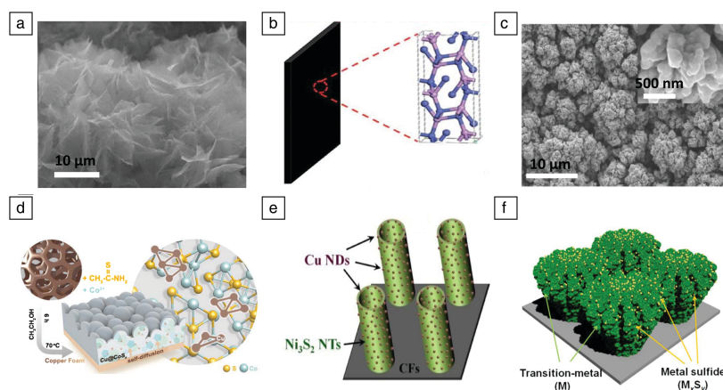
Figure 4. (a) Scanning electron microscope (SEM) image of Co/Co 3 O 4 nanosheet. 49 (b) Schematic illustration of the Co/Co 2 P electrode. The (left) Co-foil and (right) Co 2 P. Blue indicates P and purple represents Co. 47 (c) SEM image of Co/Co 2 N on a cobalt foam. The inset shows the image at a 500-nm scale. 46 (d) Schematic illustration of the synthesis of Cu/CoS x electrocatalyst via a low-temperature synthetic route involving the interdiffusion of copper species from copper foam into the CoS x film. 51 Cartoon representations of (e) Cu/Ni 3 S 2 on carbon fibers (CFs) 52 and (f) Fe/Fe 3 S 4 electrocatalyst. 53 Note: NTs, nanotubes; NDs, nanodots; M, Fe.
