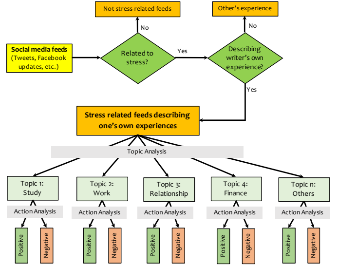
Fig. 2. Support Vector Machine (SVM) machine learning technique used to classify stress feeds by genre and topic, and assess intended actions (positive or negative) embedded in the feeds.
