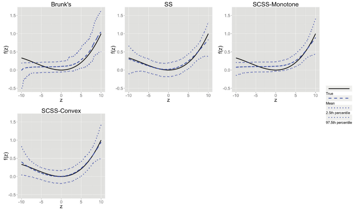
Figure A1. The estimator percentiles (2.5% and 97.5%) of SCSS for function f(x) = (20x^2 + x^3)/3000 in Example 4 under normal error.
