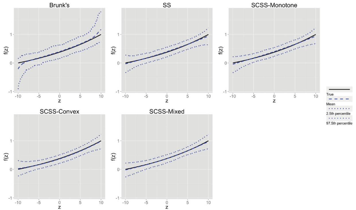
Figure A4. The estimator percentiles (2.5% and 97.5%) of SCSS for function f(x) = (e^{x/20} - e^{-10/20})/(e^{10/20} - e^{-10/20}) in Example 5 under normal error.
