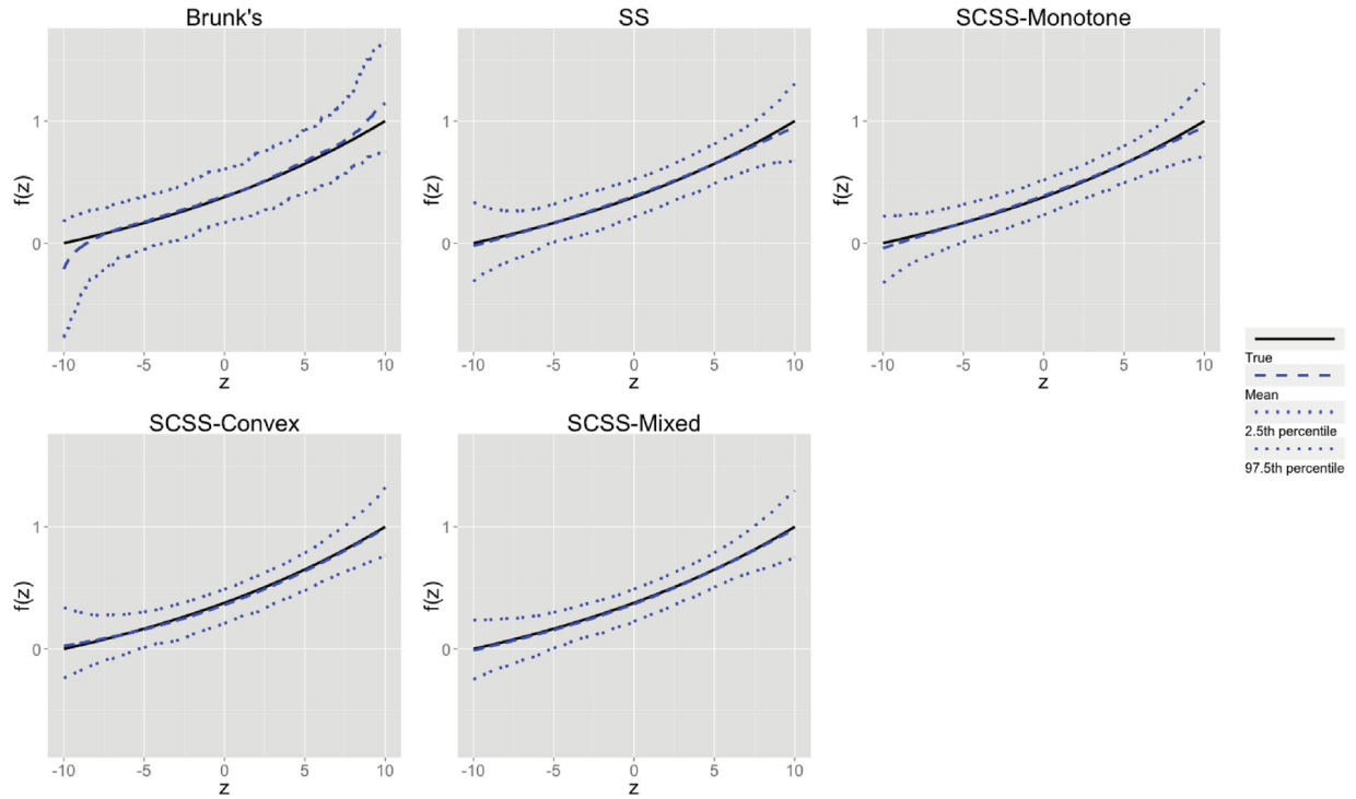
Figure A6. The estimator percentiles (2.5% and 97.5%) of SCSS for function f(x) = (e^{x/20} - e^{-10/20}) / (e^{10/20} - e^{-10/20}) in Example 5 under beta error.
