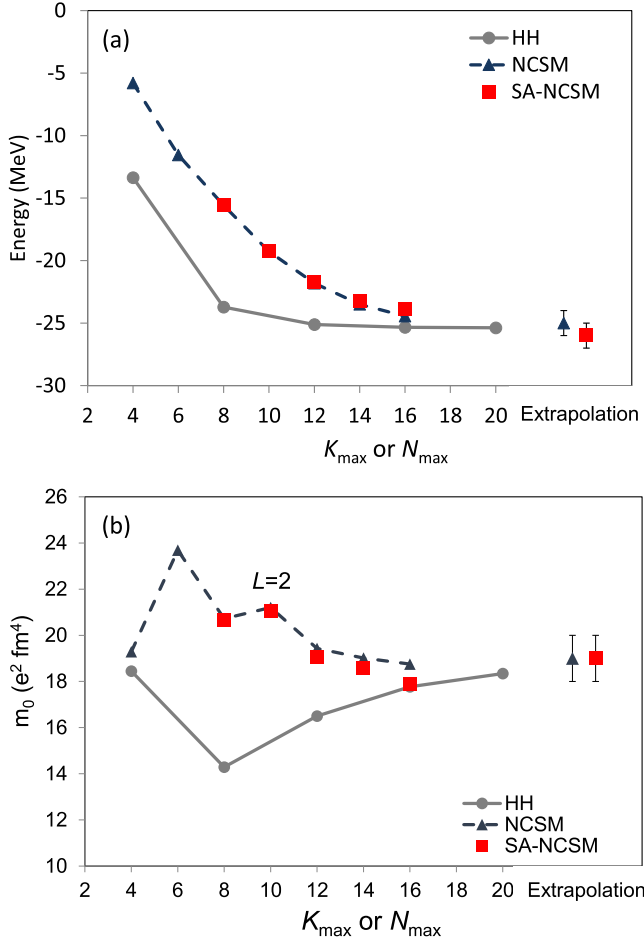
FIG. 4. (a) Ground-state energy and (b) quadrupole m_0 for ^4\text{He} using the N3LO-EM interaction (NN only) as a function of K_{\max} or N_{\max} . NCSM and SA-NCSM results are shown for \hbar\Omega = 25 MeV, while the extrapolated values are based on a range of N_{\max} (see Table I) and a 10% variation in the \hbar\Omega parameter.
