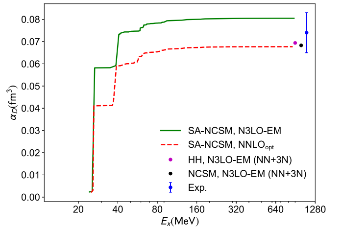
FIG. 5. Electric dipole polarizability calculated in the SA-NCSM using the N3LO-EM and \text{NNLO}_{\text{opt}} interactions (NN only) for \langle 7 | 17 model spaces and \hbar\Omega = 25 MeV. The values calculated in the HH [45] and the NCSM [59] with N3LO-EM (N3LO NN+N2LO 3N), together with the experimentally deduced value [56,57], are shown for comparison to the far right of the plot (unrelated to the E_x axis).
