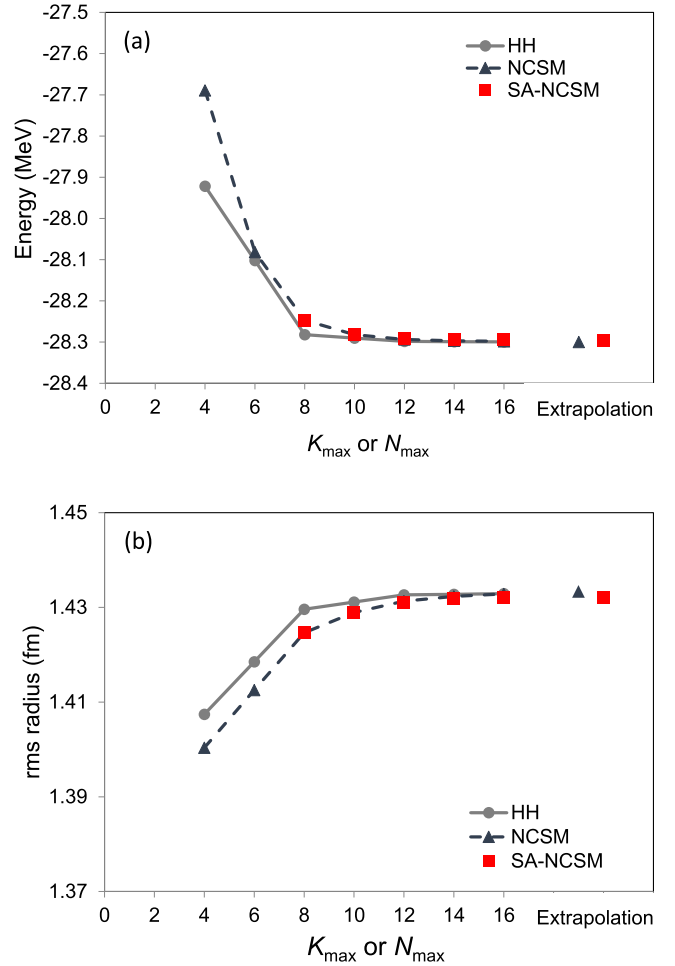
FIG. 1. (a) Ground-state energy and (b) point-proton rms radius for ^4\text{He} as a function of K_{\text{max}} or N_{\text{max}} with the JISP16 interaction. NCSM and SA-NCSM points are shown for \hbar\Omega = 25 MeV, while the extrapolated values are based on a range of N_{\text{max}} and \hbar\Omega values. Uncertainties of the extrapolated values are smaller than the size of the plot markers.
