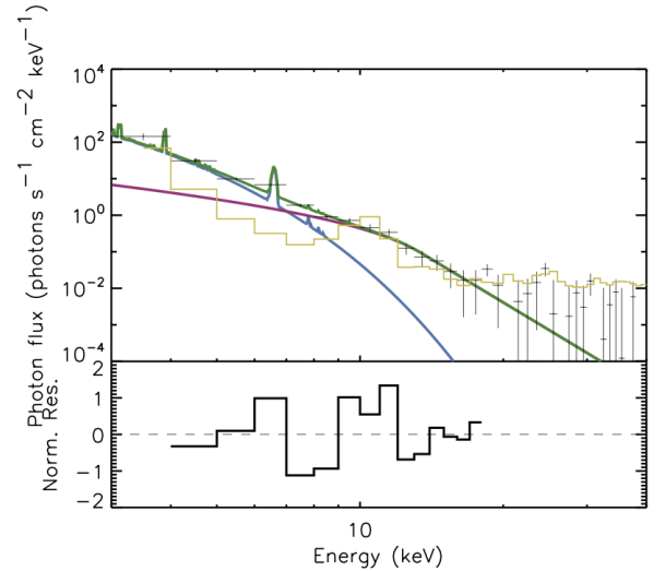
Figure 3. Top panel: RHESSI spectrum along with the fitted thermal and nonthermal components between 20:47:00 UT and 20:47:28 UT. The black crosses show the RHESSI spectrum, while the green curve shows the sum of the thermal (blue line) and nonthermal (purple line) components. The yellow histogram shows the background spectrum. Bottom panel: Normalised residuals between the spectrum and its fit.
