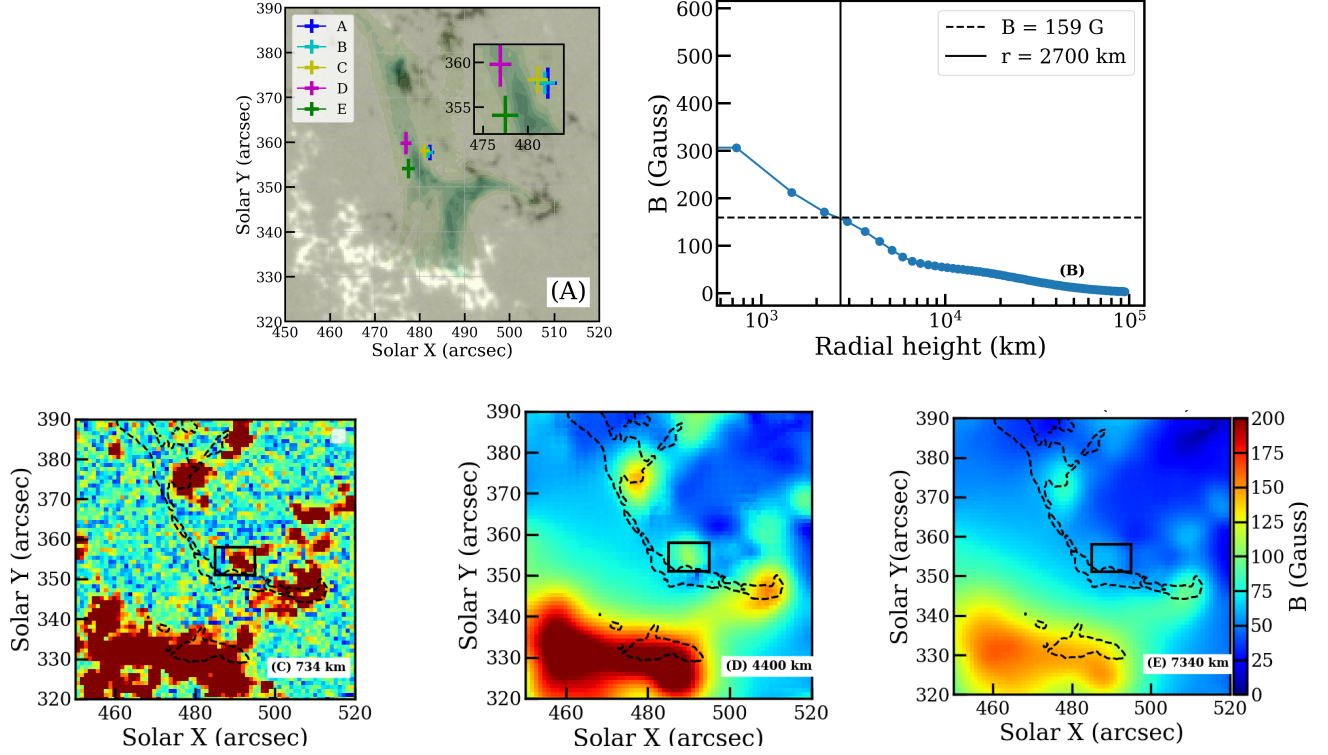
Figure 10. Panel A: Composite map of HMI magnetogram, AIA 94 Å and radio centroids of the bursts. The background black and white image is HMI magnetogram from 20:50:43 UT. The overlaid semi-transparent green image shows the AIA 94 Å map at radio burst F time. The symbol of plus marks the centroid positions of bursts from A to E. Their lengths and widths represents the 1\text{-}\sigma variation of centroid positions in frequency from 1.65 to 2.03 GHz. Panel A inset: Zoomed-in map of left panel showing variation in the radio centroid locations. Panel B: Radial profile of the maximum magnetic field in the shown rectangular region in panel C, D and E. Here dashed and solid grey lines shows the fitted magnetic field value and corresponding coronal height respectively for burst A. Panel C, D and E: Snapshots from the extrapolated 3D magnetic field configuration at different heights. The dashed-black curve shows the location of the ribbons observed in 304 Å. The solid-black rectangle marks the closest high magnetic field region ( > 200 G) to the radio sources.
