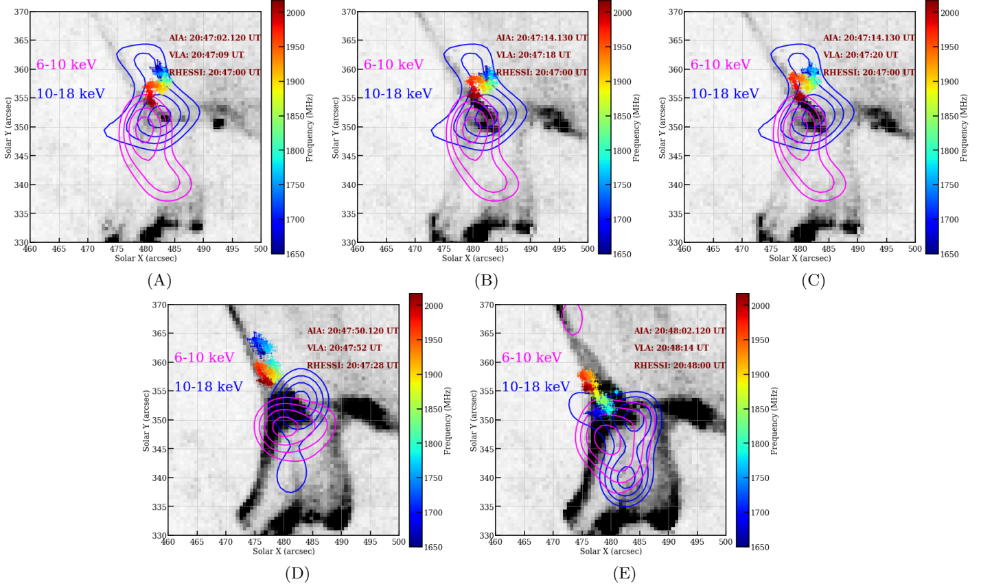
Figure 8. Evolution of the AIA 94 Å EUV ribbons (black and white image, color table inverted), X-ray RHESSI sources (magenta and blue contours) and VLA radio centroid (crosses) positions. The RHESSI contour levels are at 65%, 75%, 85% and 95% w.r.t map's peak. The AIA and RHESSI images are temporally closest to the radio bursts. The start times of AIA, VLA and RHESSI images are displayed in each panel. Note that RHESSI has an integration time of 28 sec in A, B and C, but 1 minute for D and E. The colorbar indicates the frequencies of plotted radio centroids.
