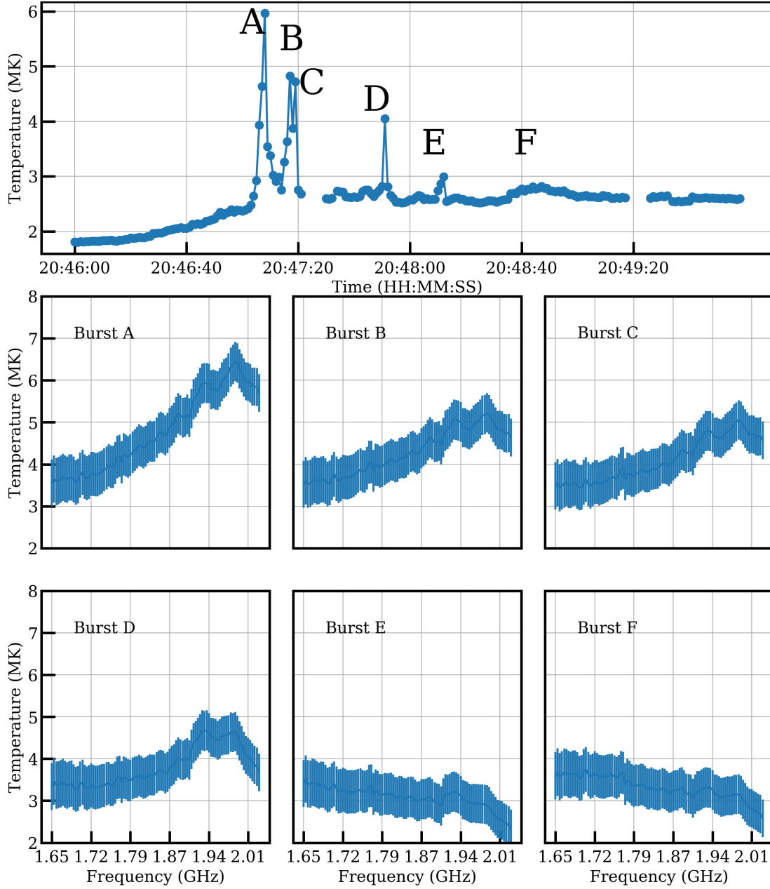
Figure 6. Top panel: Timeseries of the brightness temperature of the radio source obtained from the region corresponding to the 70% flux level at 2.0 GHz frequency in the image. Middle and lower panels: Radio spectrum for the various bursts seen in the radio source timeseries. The errorbars are the 1\text{-}\sigma variation in the image residuals.
