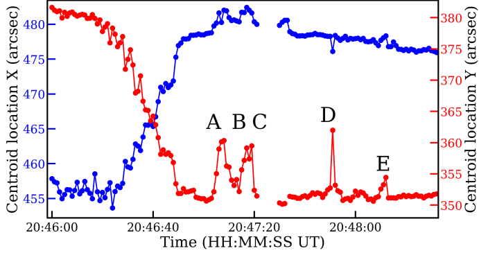
Figure 9. Centroid locations of the radio sources as function of time at 1.7 GHz. The position shifts during the burst times can be seen distinctly and are marked with letters. Note: X and Y coordinates correspond to the helioprojective solar coordinates shown in Figure 8.
