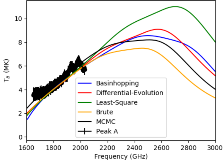
Figure 12. Fit results obtained for radio burst peak A using different algorithms. The ‘+’ plots the datapoints for radio burst A, while the colored lines are the fit for various algorithms.
