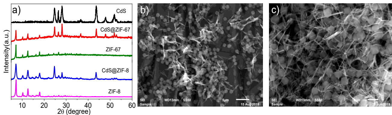
Figure 1. (a) XRD patterns of the as-prepared CdS NWs, ZIF-67, ZIF-8, CdS@ZIF-67 and CdS@ZIF-8. SEM images of CdS@ZIF-8 (b) and CdS@ZIF-67 (c).
