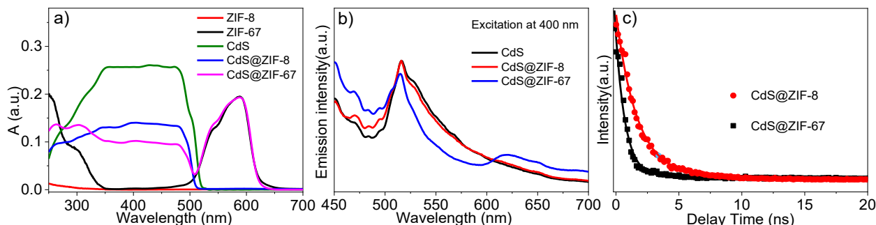
Figure 2. (a) The diffuse reflectance spectra of ZIF-8, ZIF-67, CdS NWs, CdS@ZIF-67 and CdS@ZIF-8. (b) The emission spectra of CdS NWs, CdS@ZIF-8 and CdS@ZIF-67 following 400 nm excitation. (c) The comparison of emission lifetime decay kinetics of CdS@ZIF-8 and CdS@ZIF-67 which were collected at 515 nm after 400 nm excitation. Solid lines are the fits of the decays according to equation S1.
