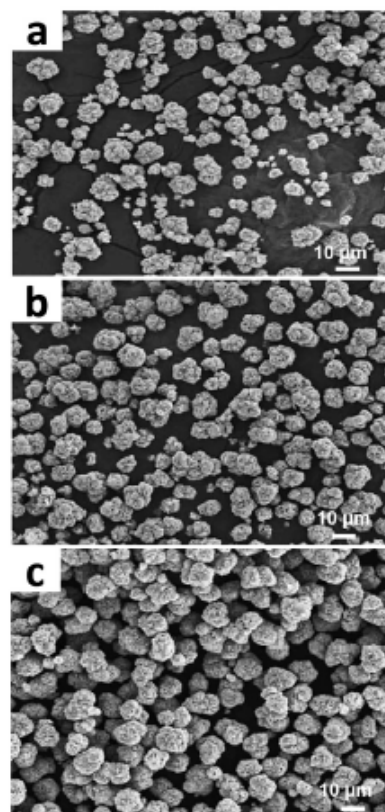
Fig. 2 SEM images of (Ni_{1/3}Co_{1/3}Mn_{1/3})(OH)_2 powders produced from hydroxide coprecipitations at various concentrations of NH_4OH as a chelating agent. a) 0.12 mol dm^{-3} NH_4OH , b) 0.24 mol dm^{-3} NH_4OH , and c) 0.36 mol dm^{-3} NH_4OH while all the other solution conditions were controlled to be the same with total TM concentration and NaOH concentration both of 2.0 mol dm^{-3} , pH of 11, stirring rate of 600 rpm in a CSTR system. Reprinted with permission from ref. 82. Copyright (2004) Elsevier.
