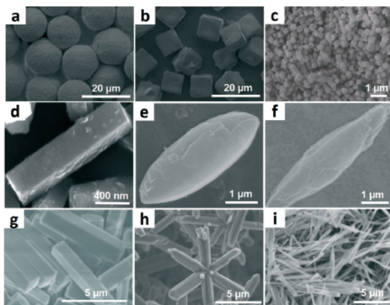
Fig. 1 Particles with different morphologies obtained from coprecipitation reactions: a) spheres, b) cubes, c) cubes, d) rods, e) ellipsoids, f) elongated ellipsoids, g) rods, h) stars, and i) needles. a and b) Reprinted with permission from ref. 51. Copyright (2015) Elsevier. c) Reprinted with permission from ref. 41. Copyright (2014) Royal Society of Chemistry. d–f) Reprinted with permission from ref. 44. Copyright (2017) American Chemical Society. g) Reprinted with permission from ref. 48. Copyright (2016) Wiley. h and i) Reprinted with permission from ref. 54. Copyright (2006) American Chemical Society.
