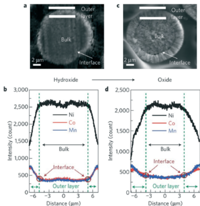
Fig. 7 Scanning electron microscopy (SEM) image (a) and electron-probe X-ray micro-analysis (EPMA) line scan results (b) of precursor hydroxide; SEM image (c) and EPMA line scan (d) of the final lithiated oxide \text{Li}[\text{Ni}_{0.64}\text{Co}_{0.18}\text{Mn}_{0.18}]\text{O}_2 . In both cases, the gradual concentration changes of Ni, Mn, and Co in the interlayer are clearly evident. The Ni concentration decreases and the Co and Mn concentrations increase towards the surface. Reprinted with permission from ref. 2.
