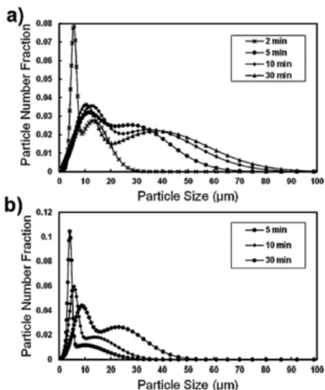
Fig. 6 Particle size distributions at 5, 10, and 30 min after the start of the precipitation in a) manganese oxalate, b) nickel oxalate coprecipitations. Solid lines added to guide the eye. Reprinted with permission from ref. 140. Copyright (2018) Elsevier.
