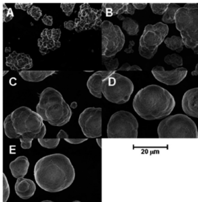
Fig. 5 SEM images of \text{Ni}(\text{OH})_2 harvested from the same coprecipitation reactions after A) 2 hours, B) 5 hours, C) 10 hours, D) 15 hours, and E) 20 hours. Reprinted with permission from ref. 52. Copyright (2009) American Chemical Society.
