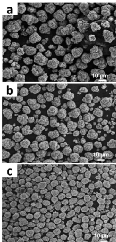
Fig. 3 SEM images of (\text{Ni}_{1/3}\text{Co}_{1/3}\text{Mn}_{1/3})(\text{OH})_2 powders produced from hydroxide coprecipitations at various stirring speeds. a) 400 rpm, b) 800 rpm, and c) 1000 rpm while all the other solution conditions were controlled to be the same with total TM concentration and NaOH concentration both of 2.0 \text{ mol dm}^{-3} , pH of 11, and 0.36 \text{ mol dm}^{-3} \text{NH}_4\text{OH} in a CSTR system. Reprinted with permission from ref. 82. Copyright (2004) Elsevier.
