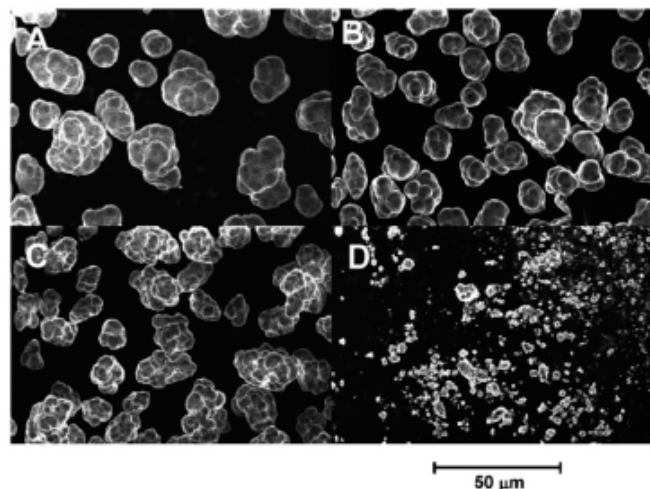
Fig. 4 SEM images of \text{Ni(OH)}_2 particles synthesized from coprecipitation reactions with a pH value of A) 10.6, B) 11.0, C) 11.4, and D) 11.8 while other solution conditions were controlled the same in a continuous system. Reprinted with permission from ref. 52. Copyright (2009) American Chemical Society.
