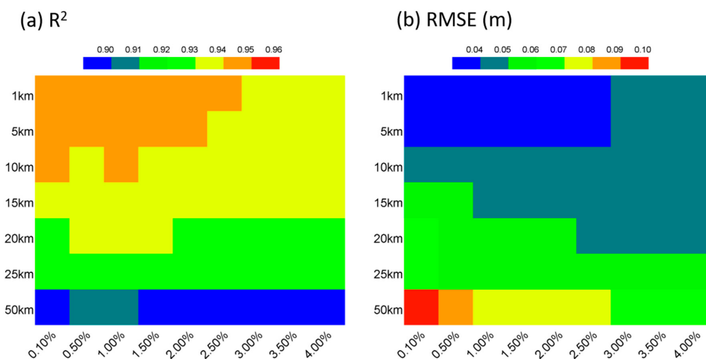
Figure 9. The R^2 (a) and RMSE (m) (b) for all the tracks combined between retrievals from the lowest elevation method and retrievals from the DMS method (ground truth) at 7 segment length scales: 1, 5, 10, 15, 20, 25, and 50 km, for 9 percentage scales: 0.1%, 0.5%, 1%, 1.5%, 2%, 2.5%, 3%, 3.5%, and 4% (the x-axis).
