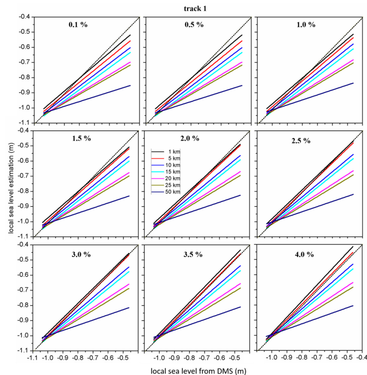
Figure 3. Linear fit lines of track 1 between retrievals from the lowest elevation method and those from the DMS method (ground truth) at 7 segment length scales: 1, 5, 10, 15, 20, 25, and 50 km, and 9 percentage scales: 0.1%, 0.5%, 1%, 1.5%, 2%, 2.5%, 3%, 3.5%, and 4%. The dashed line is the 1:1 line. All linear least square fits are statistically significant with greater than 95% confidence using an F test.
