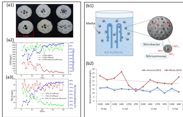
Fig. 5 3D-printed biocarriers with various structures. (a) 3-D printed honeycomb spherical biocarriers consisted of pentahedrons and hexahedrons: (a1) Images and treatment efficiencies of (a2) COD & (a3) Ammonia; Reproduced with permission from ref. 122. Copyright © 2015 Springer Nature. (b) Biocarriers made of 3-D printed acrylate polymer with spherical gyroid structures: (b1) images and schemes of bioreactor and (b2) treatment results of simulated wastewater that contained ammonia and nitrate. Reproduced with permission from ref. 123. Copyright © 2017 John Wiley and Sons.
