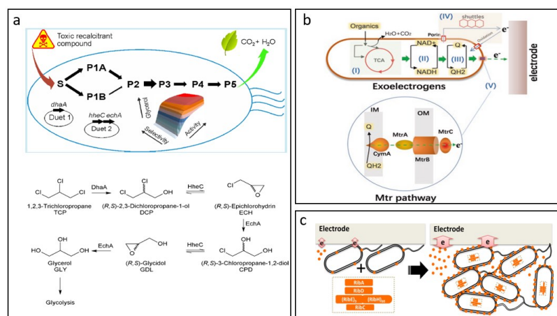
Fig. 4 Engineering biological pathways to enhance metabolism-driven pollutants removal. (a) Top: Schematic illustration of toxic compound is degraded into nontoxic, clean product through pre-designed metabolic pathway. Bottom: The synthetic pathway for the biodegradation of TCP assembled in E. coli into glycol. Reproduced with permission from ref. 83. Copyright © 2014, American Chemical Society. (b) Five modules in electroactive bacteria for EET. (I) The oxidation of organics (initial electron donor) and TCA cycle; (II) the redox of NADH; (III) the redox of quinone pool; (IV) electron transfer to extracellular electrode by shuttles through porin complex; and (V) the representative Shewanella metal-reducing (Mtr) pathway for EET. Reproduced with permission from ref. 85. Copyright © 2019, Springer Nature Singapore Pte Ltd. (c) Synthetic flavin biosynthesis pathway from Bacillus subtilis was heterologously expressed in S. oneidensis MR-1, resulting in ~25.7 times' increase in secreted flavin concentration and enhanced EET performance. Reproduced with permission from ref. 87. Copyright © 2015, American Chemical Society.
