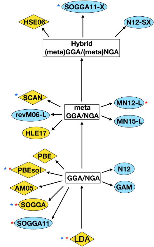
FIG. 1. Jacob's Ladder diagram describing the functionals that are investigated in this work. The functionals in diamonds are the standard representative(s) in each rung, while those in ovals are the Minnesota ones. Yellow shading indicates functionals that have been previously used on ferroelectrics, while blue shading indicates those that have not been tested. Blue (red) asterisks denote the best-performing functionals found in this study for the case of BTO (PTO), respectively.
