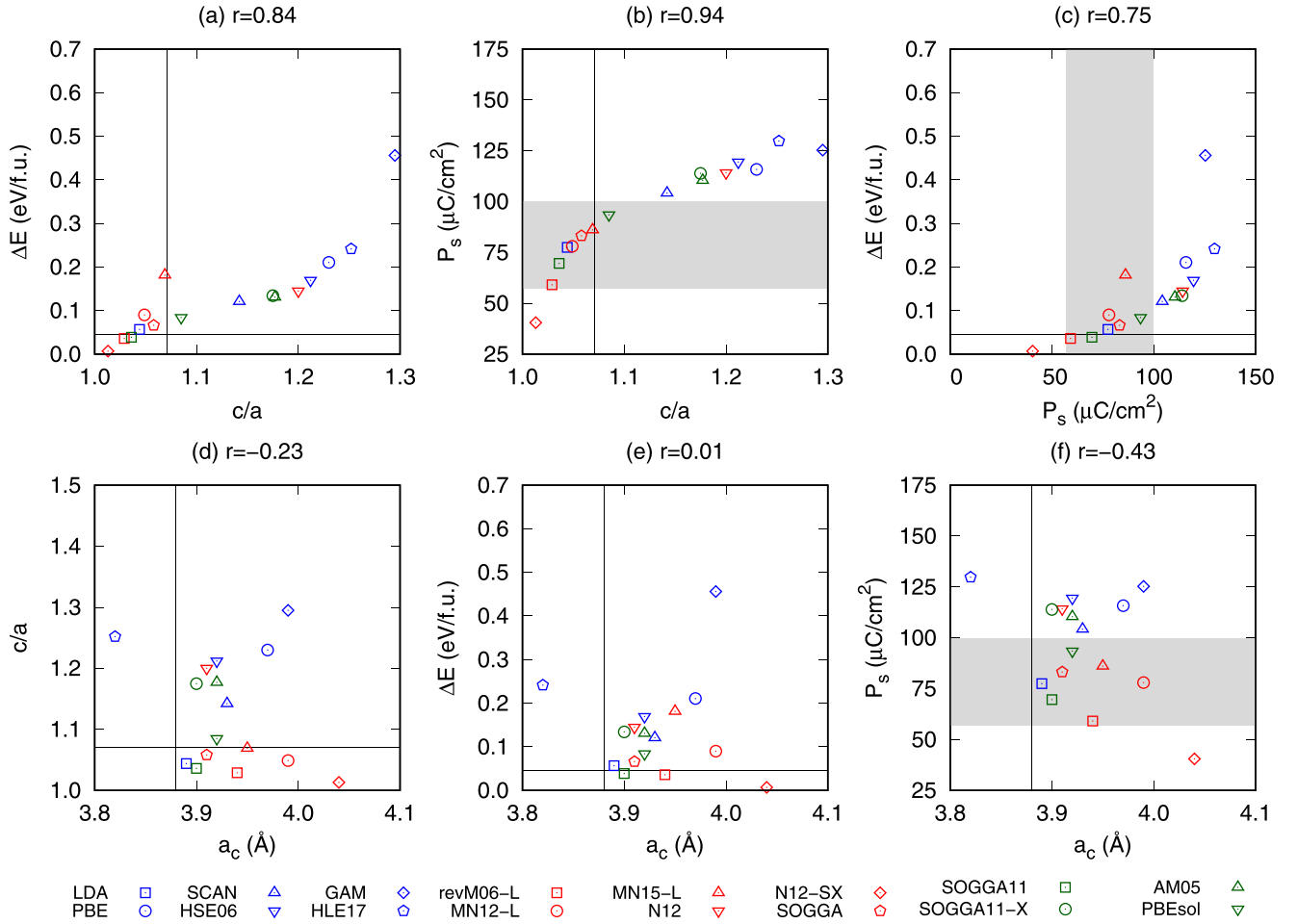
FIG. 4. Correlation plots for PTO. The correlation coefficient r is given above each graph. Experimental data are taken from Refs. [1], [2], [37], and [38].
