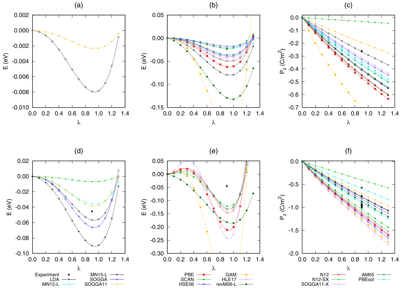
FIG. 2. Energy (a, b, d, e) and polarization (c, f) along the distortion path for BTO and PTO, respectively. Shallow energy wells (a, d); deeper wells (b, e). Experimental data for BTO are taken from Refs. [1], [2], [50], and [52]. Experimental data for PTO are taken from Refs. [1], [50], [55], and [56]. Note that the GAM data are outside of plotting range.
